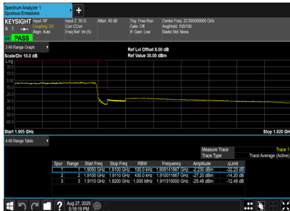
N2(40M)_DFT-s- OFDM_BPSK_Outer_Full_High_CH
