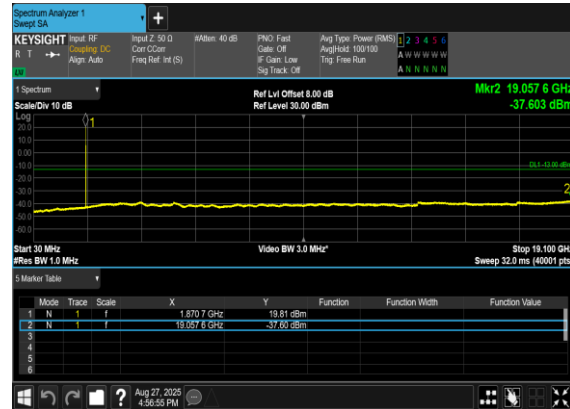
N2(20M)_DFT-s- OFDM_QPSK_Edge_1RB_Left_Mid_CH
