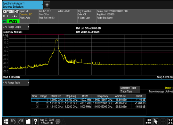
N2(40M)_DFT-s- OFDM_BPSK_Edge_1RB_Right_High_CH
