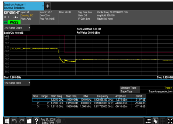
N2(40M)_DFT-s- OFDM_QPSK_Outer_Full_High_CH
