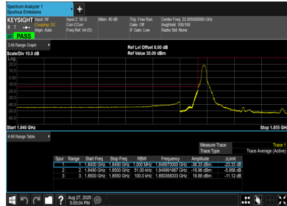
N2(5M)_DFT-s- OFDM_QPSK_Edge_1RB_Left_Low_CH
