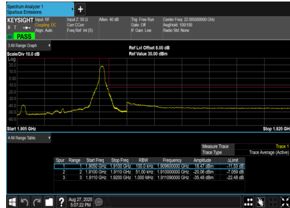
N2(5M)_DFT-s- OFDM_QPSK_Edge_1RB_Right_High_CH
