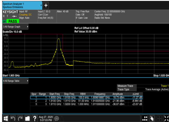
N2(5M)_DFT-s- OFDM_BPSK_Edge_1RB_Right_High_CH
