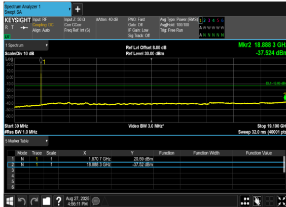
N2(20M)_DFT-s- OFDM_BPSK_Edge_1RB_Left_Mid_CH
