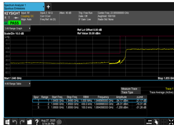
N2(40M)_DFT-s- OFDM_QPSK_Outer_Full_Low_CH
