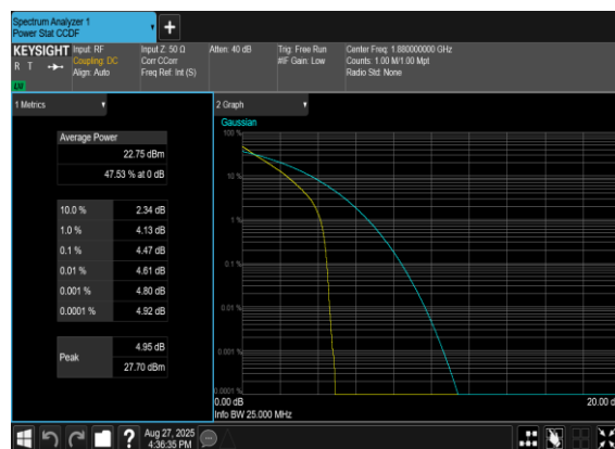
N2(20M)_DFT-s- OFDM_QPSK_Outer_Full_Mid_CH
