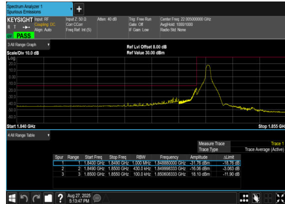
N2(40M)_DFT-s- OFDM_QPSK_Edge_1RB_Left_Low_CH
