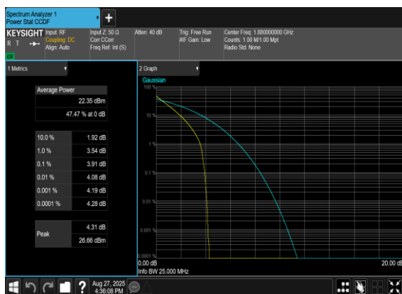
N2(20M)_DFT-s-OFDM_PI_2- BPSK_Outer_Full_Mid_CH
