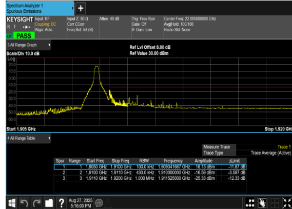
N2(40M)_DFT-s- OFDM_QPSK_Edge_1RB_Right_High_CH
