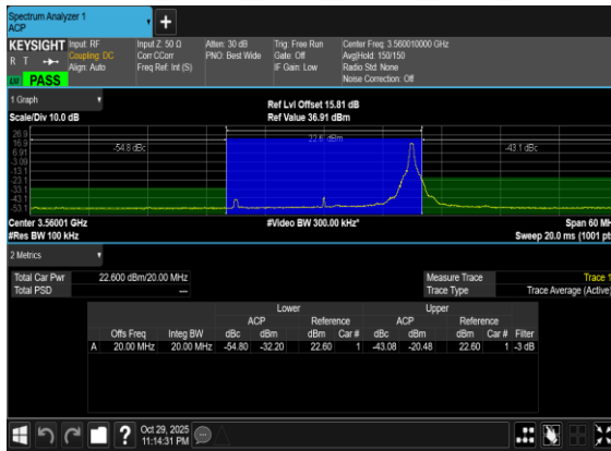
N48(20M)_DFT-s-OFDM_PI_2- BPSK_Edge_1RB_Right_Low_CH
