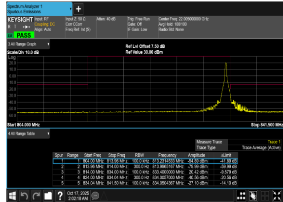
N26(20M)_DFT-s- OFDM_QPSK_Edge_1RB_Right_Mid_CH
