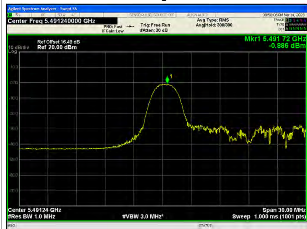
PSD NVNT ax20 26@0 5500MHz Ant3
