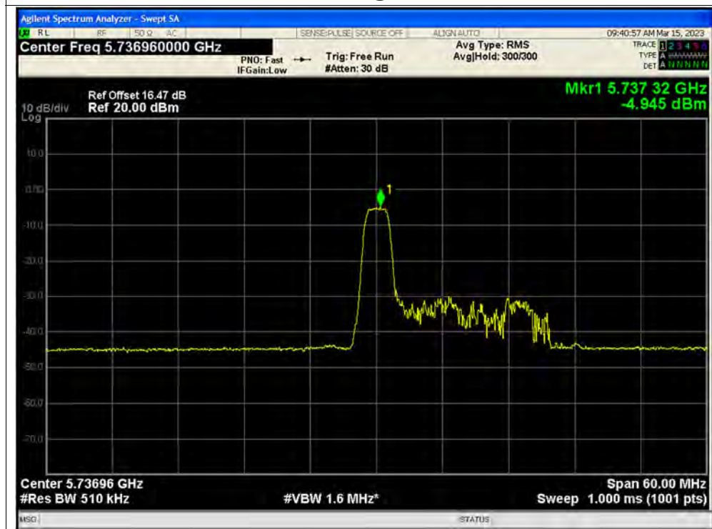
PSD NVNT ax40 26@0 5755MHz Ant3
