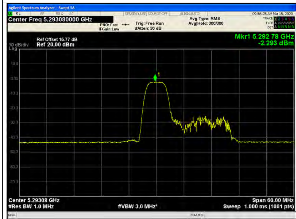
PSD NVNT ax40 52@37 5310MHz Ant3
