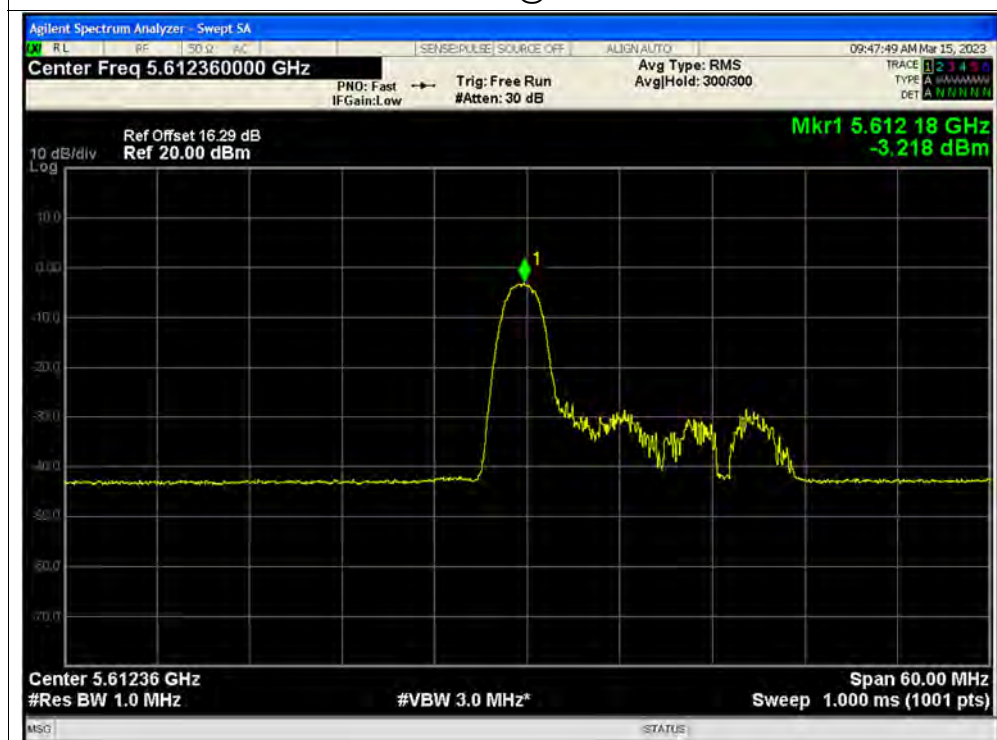
PSD NVNT ax40 26@0 5630MHz Ant3
