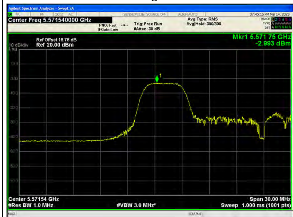
PSD NVNT ax20 52@37 5580MHz Ant3
