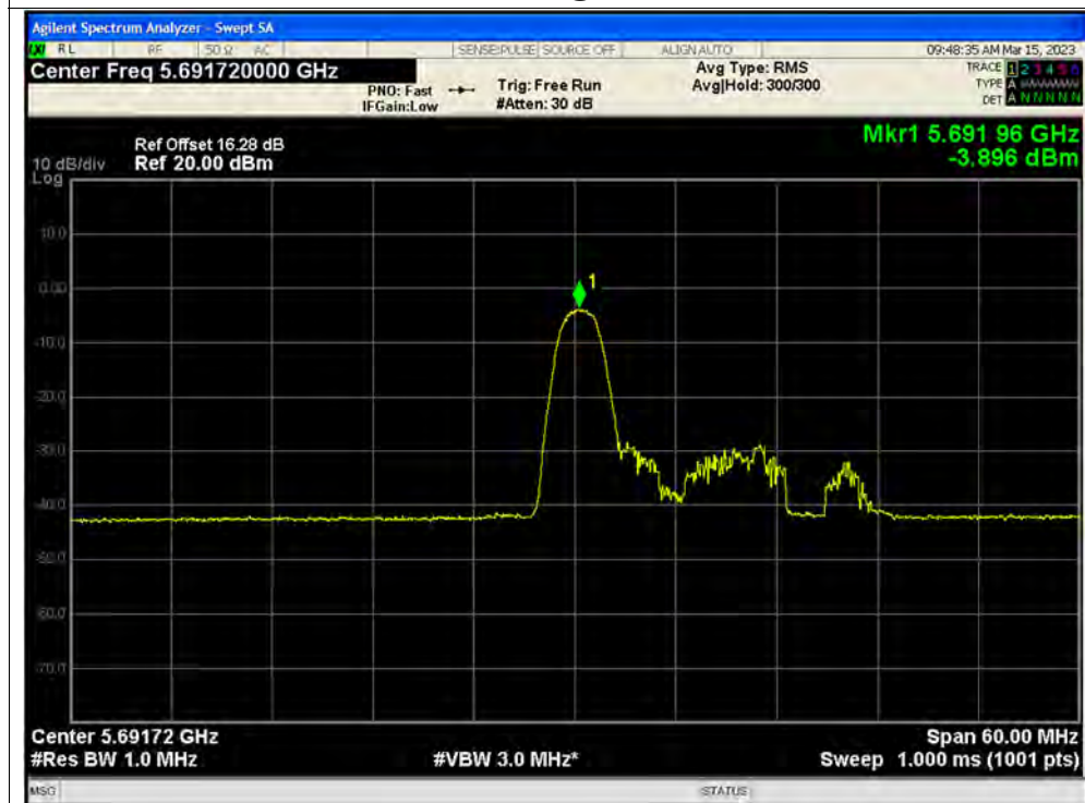
PSD NVNT ax40 26@0 5710MHz Ant3
