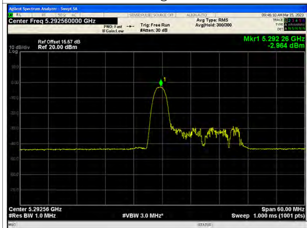
PSD NVNT ax40 26@0 5310MHz Ant3
