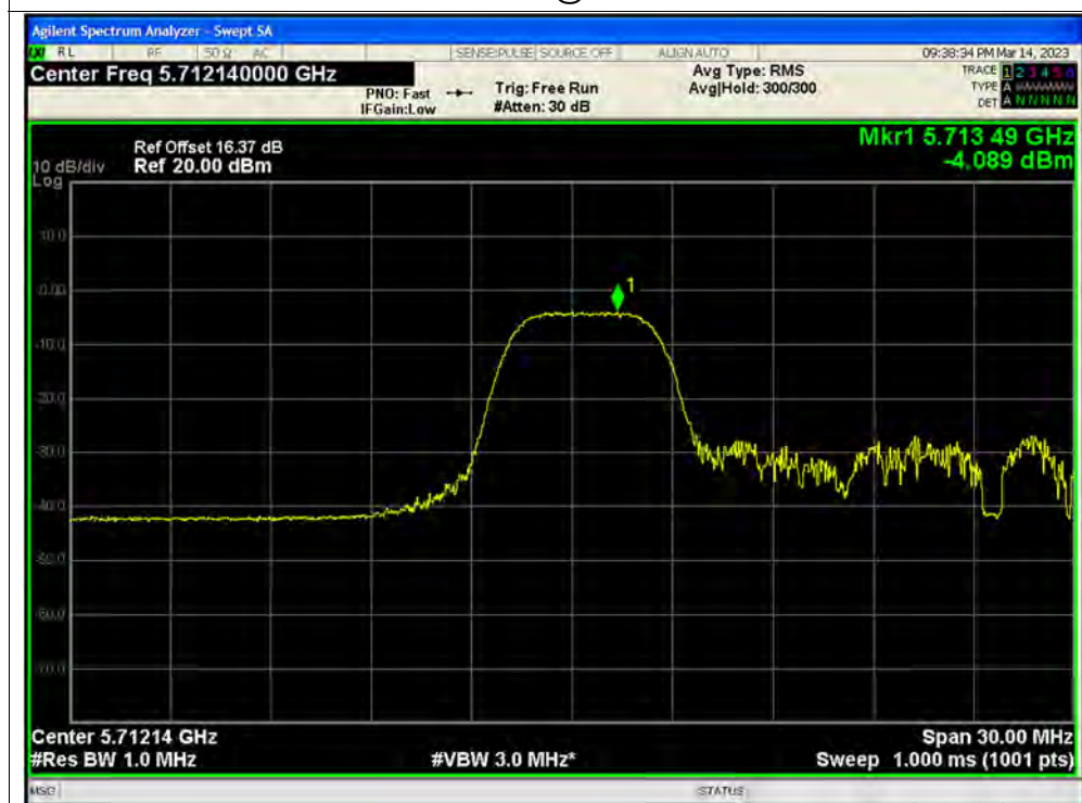
PSD NVNT ax20 52@37 5720MHz Ant3
