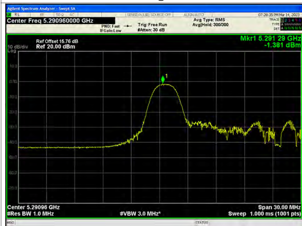
PSD NVNT ax20 26@0 5300MHz Ant3
