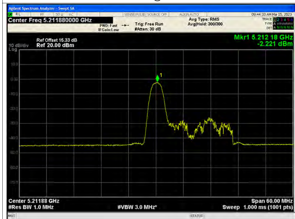
PSD NVNT ax40 26@0 5230MHz Ant3
