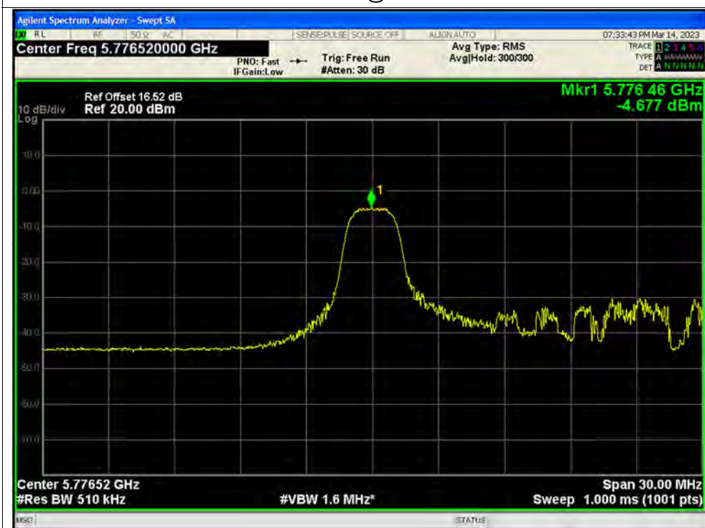
PSD NVNT ax20 26@0 5785MHz Ant3
