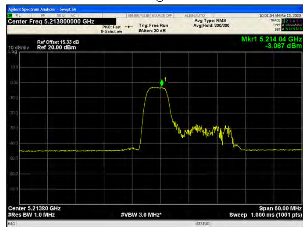
PSD NVNT ax40 52@37 5230MHz Ant3
