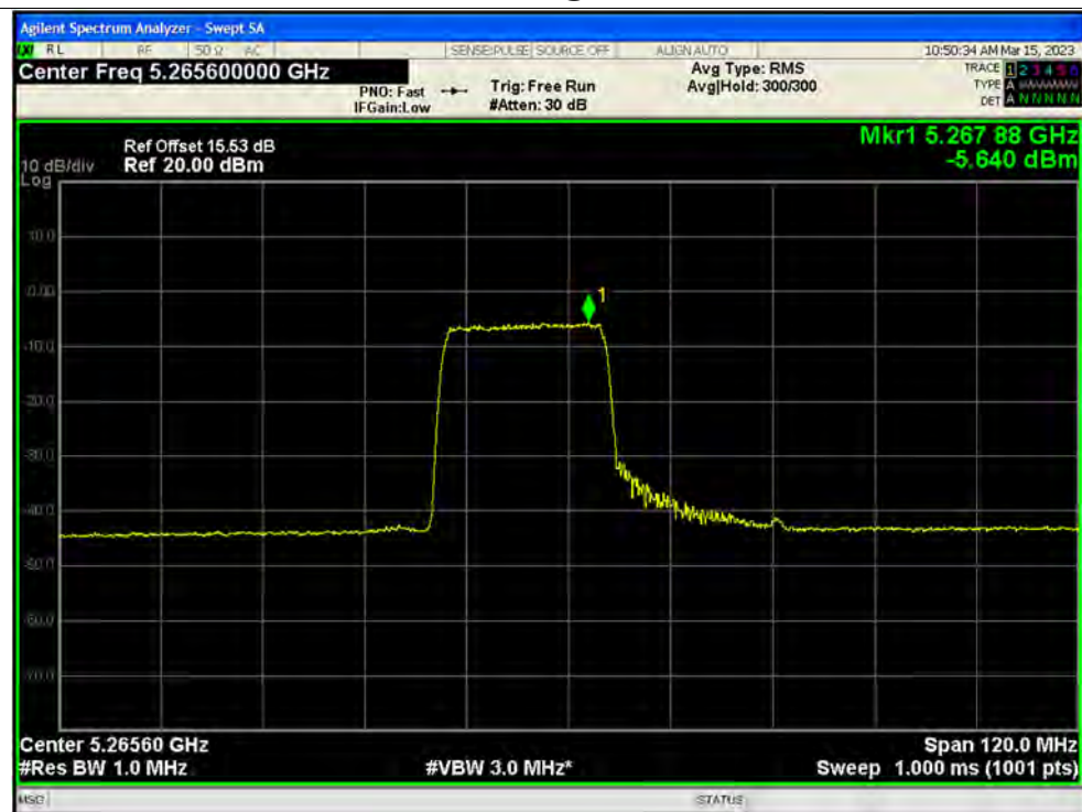
PSD NVNT ax80 242@61 5290MHz Ant3
