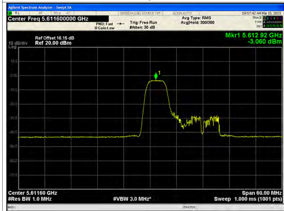
PSD NVNT ax40 52@37 5630MHz Ant3
