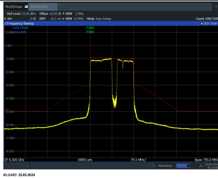
11BE160MIMO_Ant1_6505_996+484+242_Non-OFDMA_6
