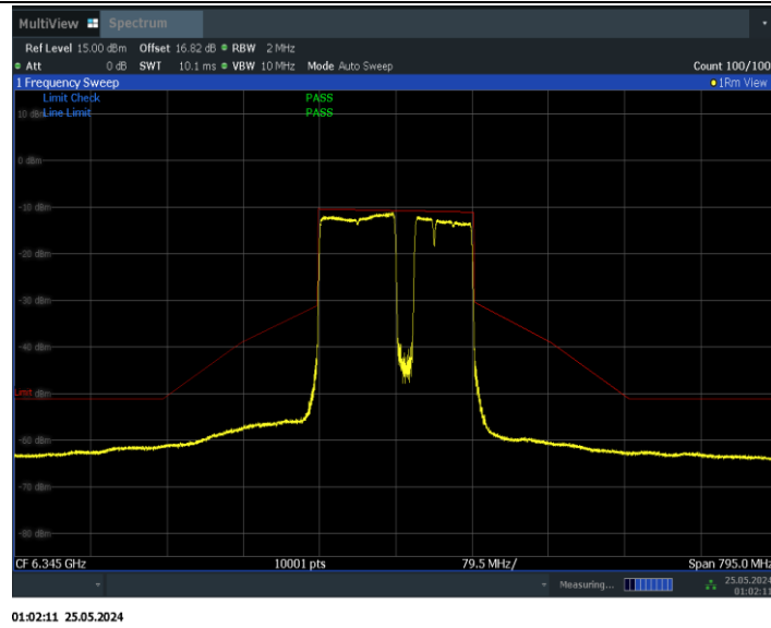
11BE160MIMO_Ant0_6345_996+484+242_Non-OFDMA_7
