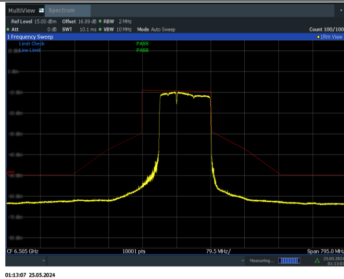
11BE160MIMO_Ant1_6505_996+484+242_Non-OFDMA_1
