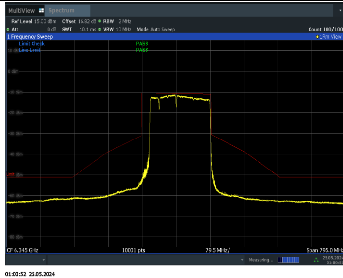
11BE160MIMO_Ant0_6345_996+484+242_Non-OFDMA_2
