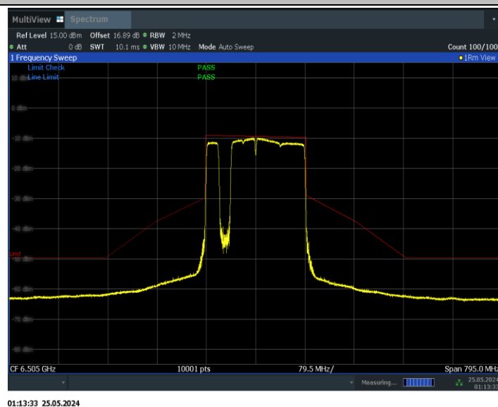
11BE160MIMO_Ant1_6505_996+484+242_Non-OFDMA_2
