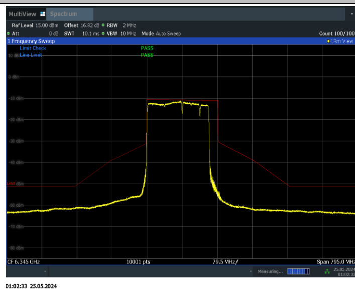
11BE160MIMO_Ant0_6345_996+484+242_Non-OFDMA_8
