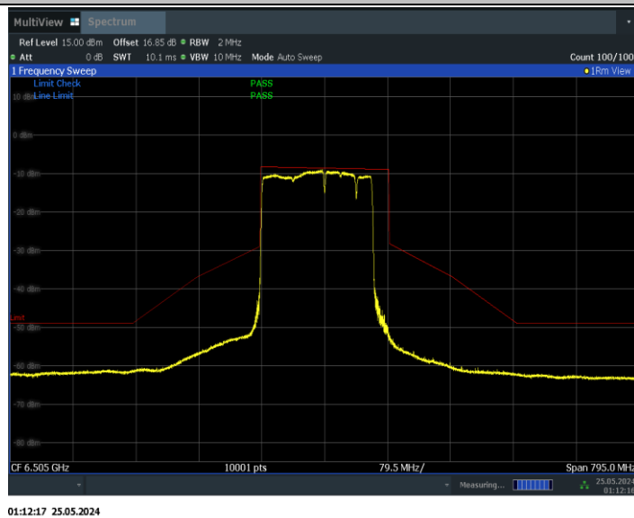
11BE160MIMO_Ant1_6505_996+484_Non-OFDMA_1
