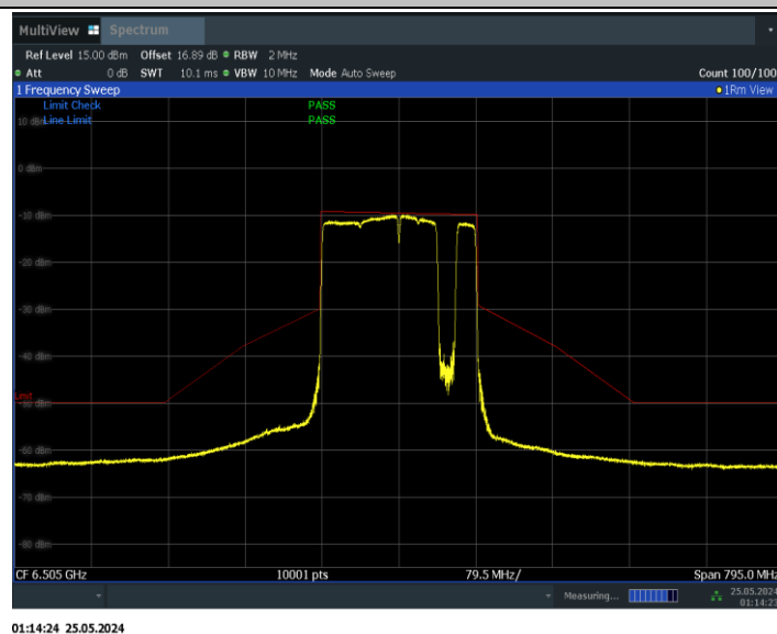
11BE160MIMO_Ant1_6505_996+484+242_Non-OFDMA_7
