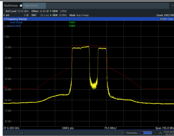
11BE160MIMO_Ant1_6505_996+484_Non-OFDMA_2
