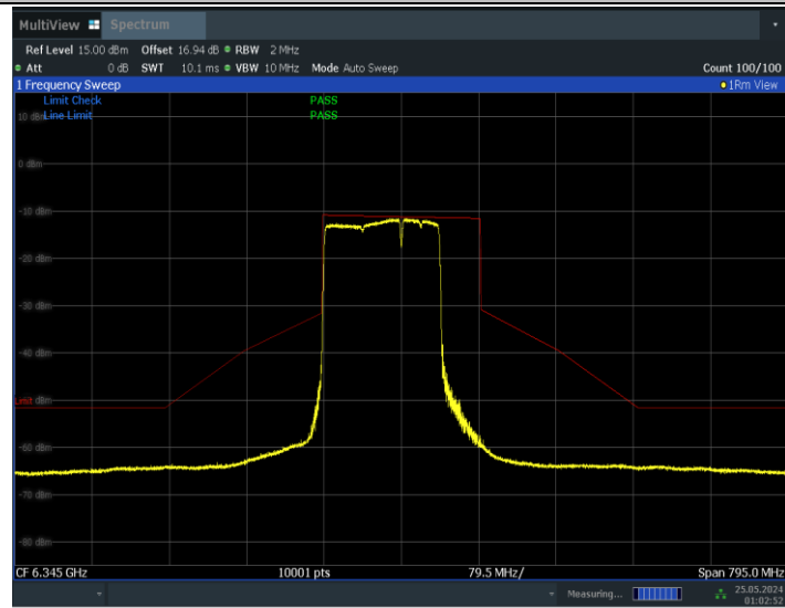
11BE160MIMO_Ant1_6345_996+484_Non-OFDMA_1
