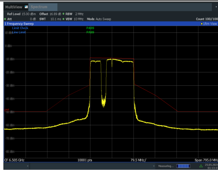
11BE160MIMO_Ant1_6505_996+484+242_Non-OFDMA_3
