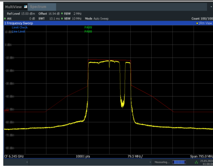
11BE160MIMO_Ant1_6345_996+484+242_Non-OFDMA_7
