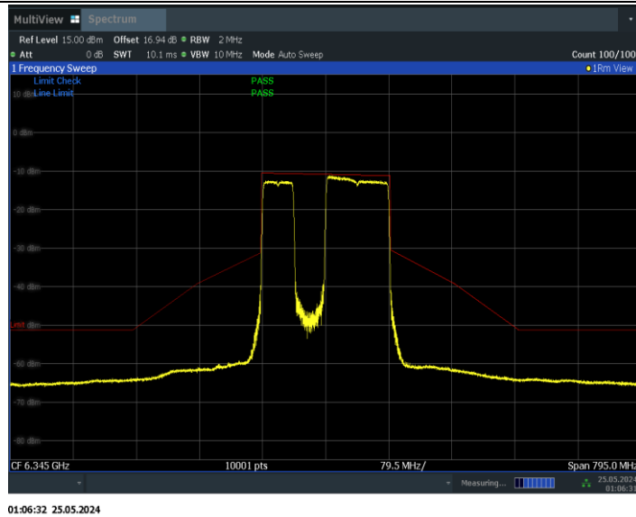
11BE160MIMO_Ant1_6345_996+484_Non-OFDMA_4
