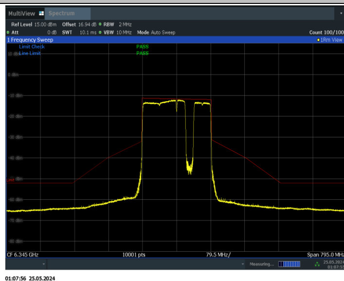
11BE160MIMO_Ant1_6345_996+484+242_Non-OFDMA_6
