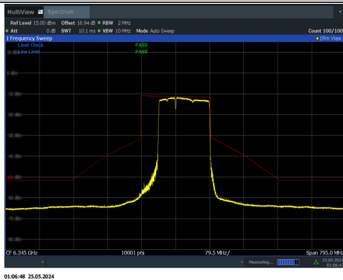
11BE160MIMO_Ant1_6345_996+484+242_Non-OFDMA_1
