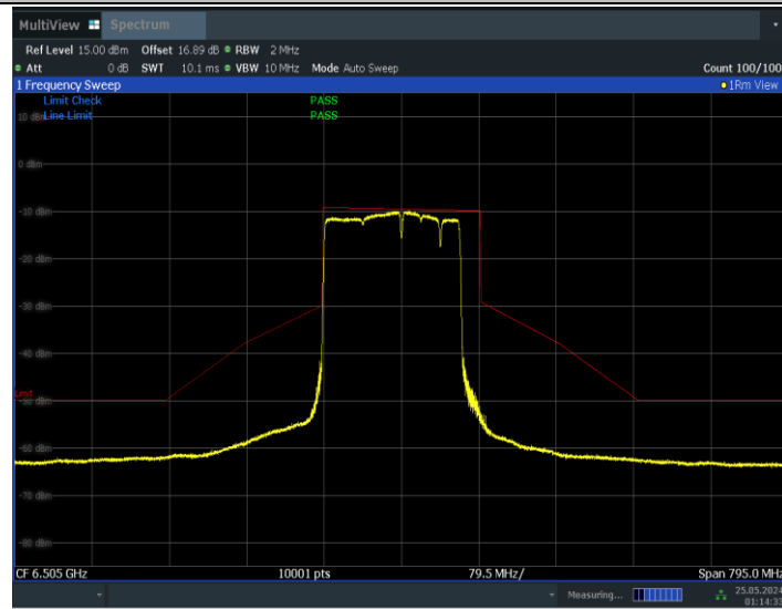
11BE160MIMO_Ant1_6505_996+484+242_Non-OFDMA_8
