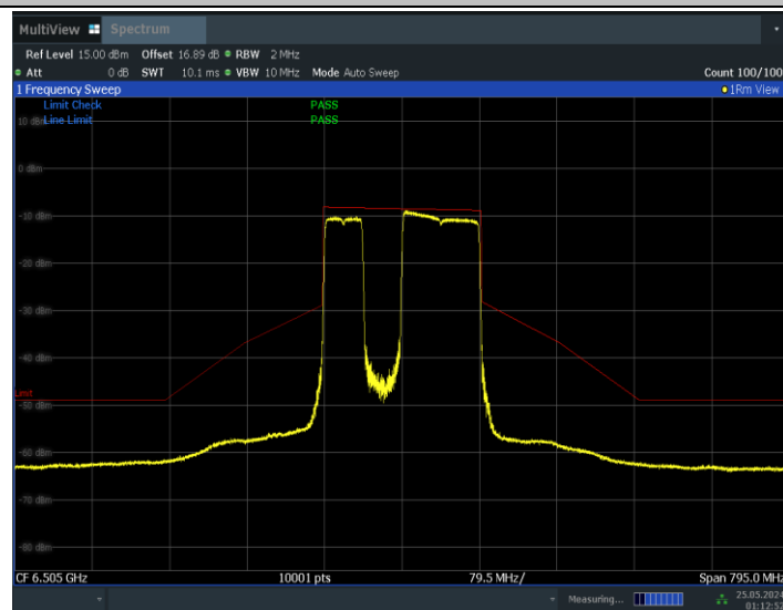
11BE160MIMO_Ant1_6505_996+484_Non-OFDMA_3
