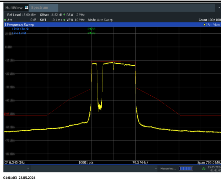
11BE160MIMO_Ant0_6345_996+484+242_Non-OFDMA_3
