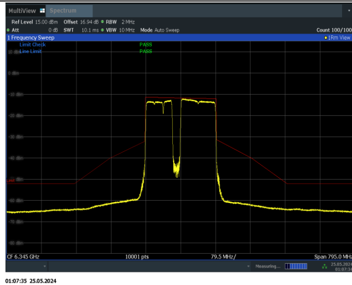
11BE160MIMO_Ant1_6345_996+484+242_Non-OFDMA_5
