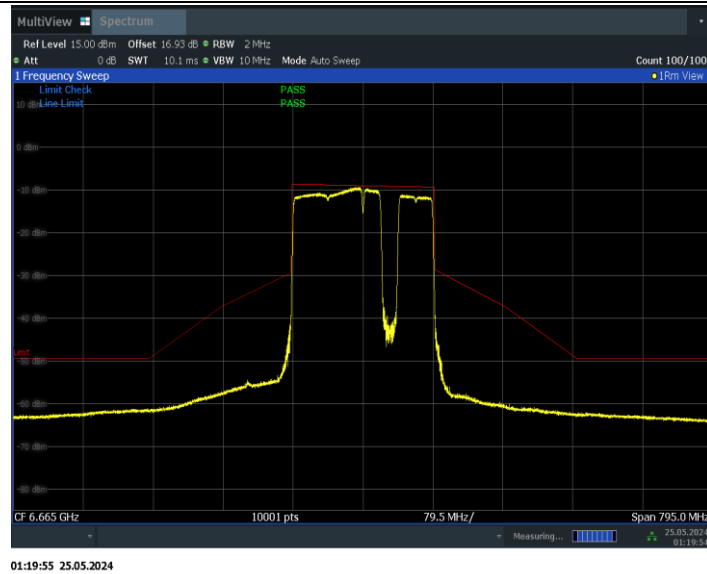
11BE160MIMO_Ant1_6665_996+484+242_Non-OFDMA_7
