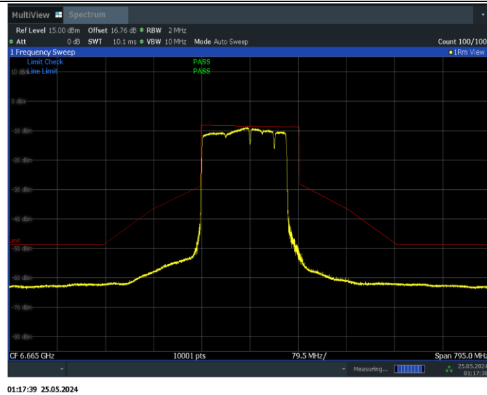
11BE160MIMO_Ant1_6665_996+484_Non-OFDMA_1
