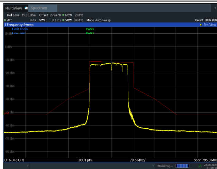
11BE160MIMO_Ant1_6345_996+484+242_Non-OFDMA_8
