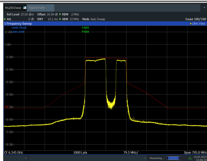
11BE160MIMO_Ant1_6345_996+484_Non-OFDMA_2
