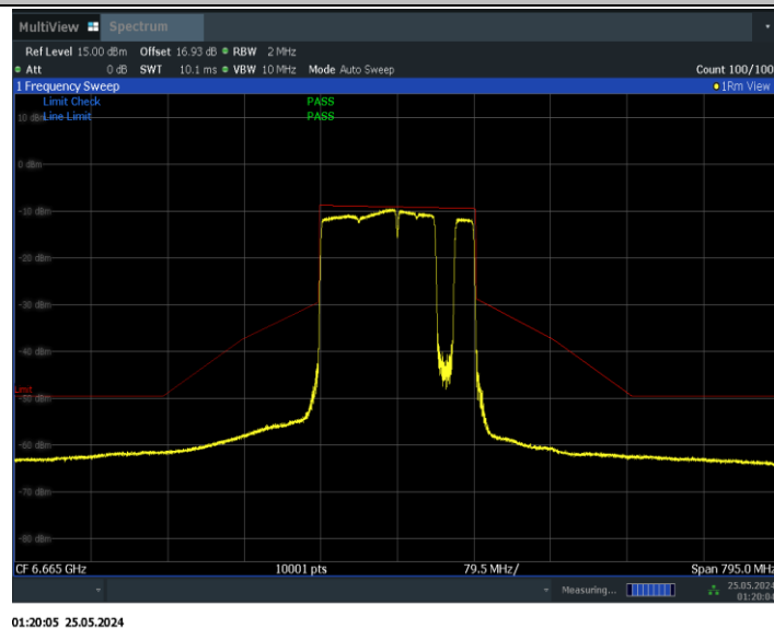
11BE160MIMO_Ant1_6665_996+484+242_Non-OFDMA_8
