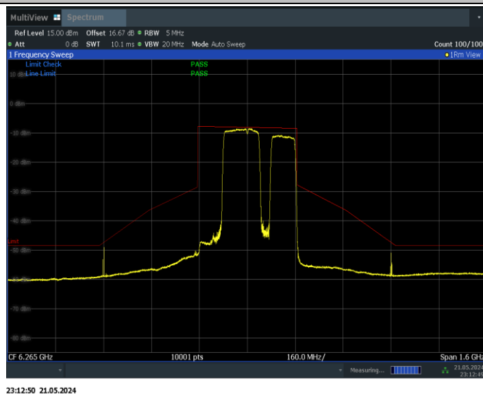
11BE320MIMO_Ant1_6265_2*996+484_Non-OFDMA_10
