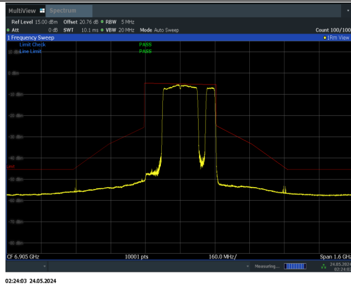
11BE320MIMO_Ant1_6905_2*996+484_Non-OFDMA_12
