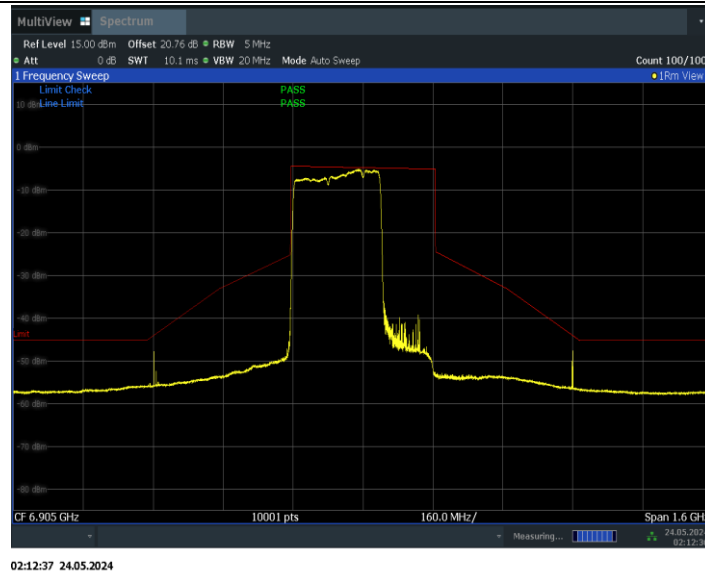
11BE320MIMO_Ant1_6905_2*996+484_Non-OFDMA_7
