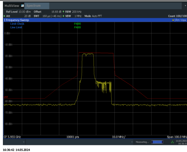
11BE20MIMO_Ant1_5955_106+26_OFDMA_1
