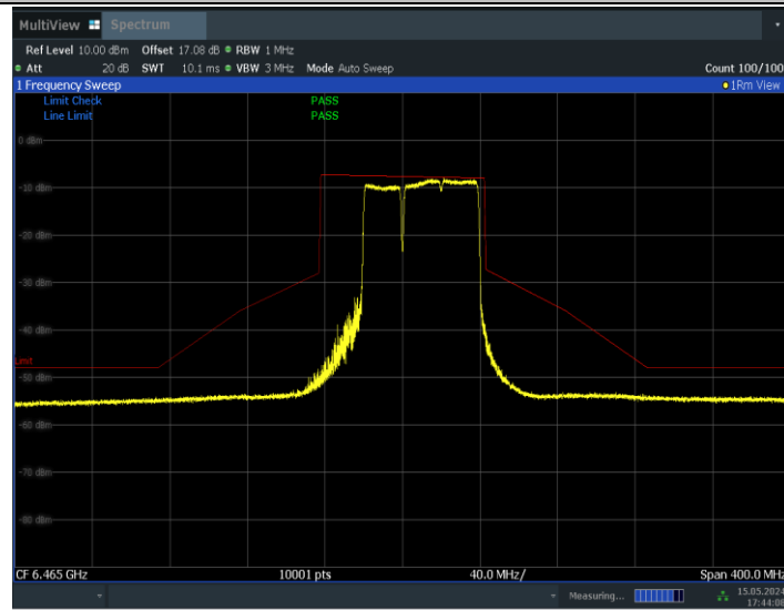
11BE80MIMO_Ant1_6465_484+242_Non-OFDMA_1
