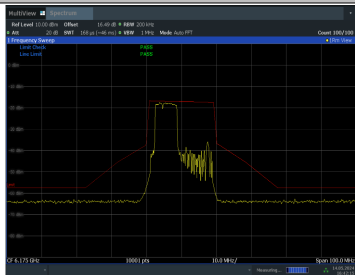
11BE20MIMO_Ant1_6175_52+26_OFDMA_1
