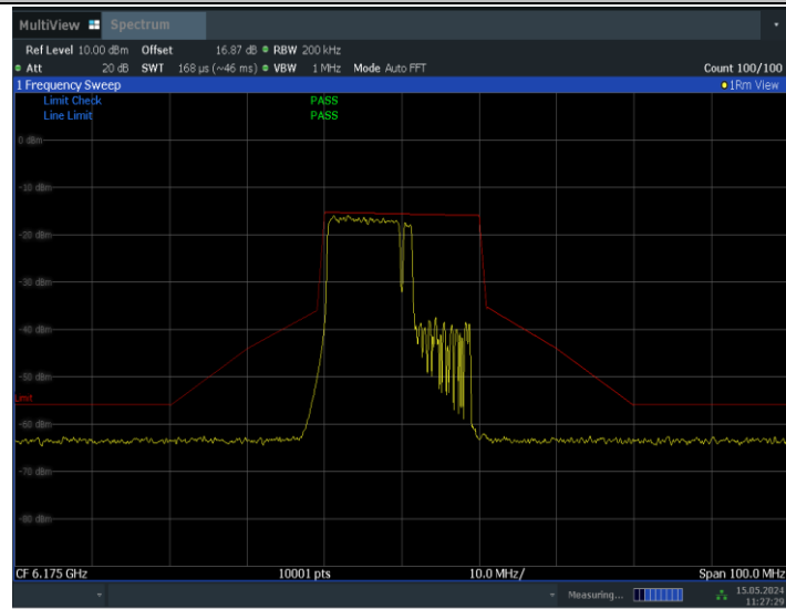
11BE20MIMO_Ant0_6175_106+26_OFDMA_1
