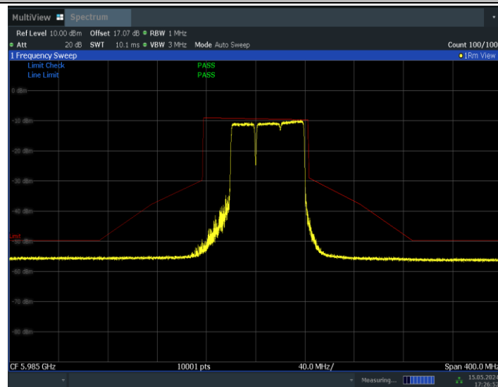
11BE80MIMO_Ant1_5985_484+242_Non-OFDMA_1
