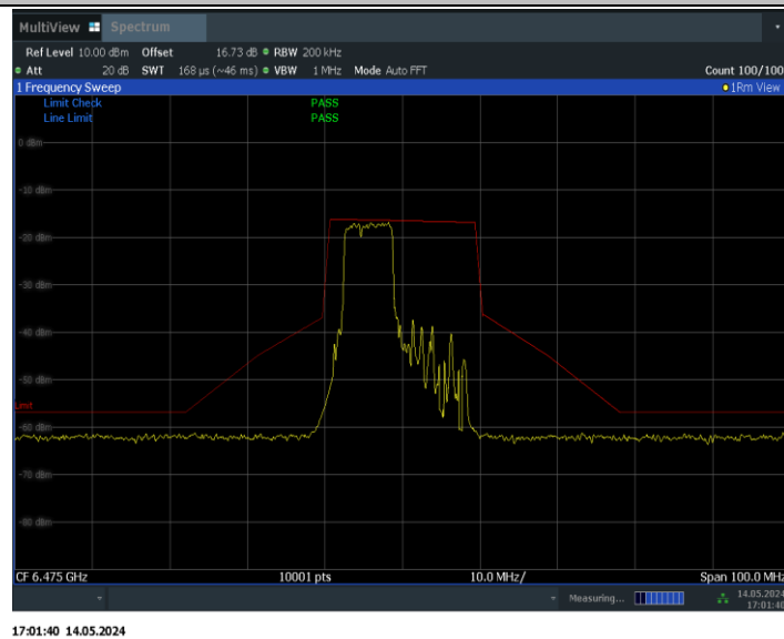
11BE20MIMO_Ant1_6475_106+26_OFDMA_1
