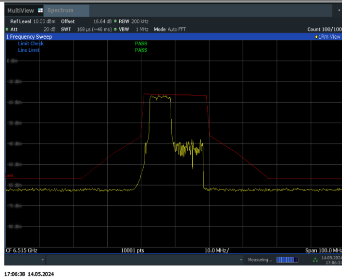
11BE20MIMO_Ant1_6515_106+26_OFDMA_1
