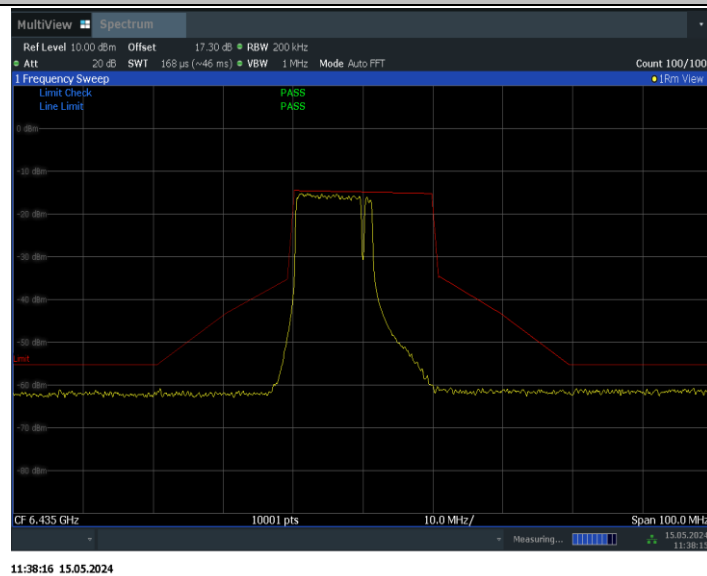
11BE20MIMO_Ant1_6435_52+26_OFDMA_1
