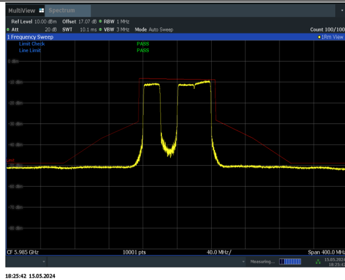
11BE80MIMO_Ant1_5985_484+242_Non-OFDMA_3
