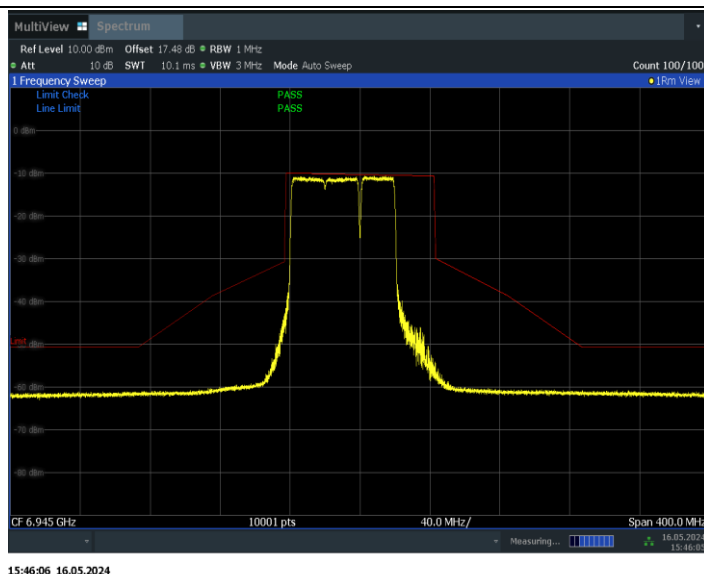
11BE80MIMO_Ant1_6945_484+242_Non-OFDMA_1
