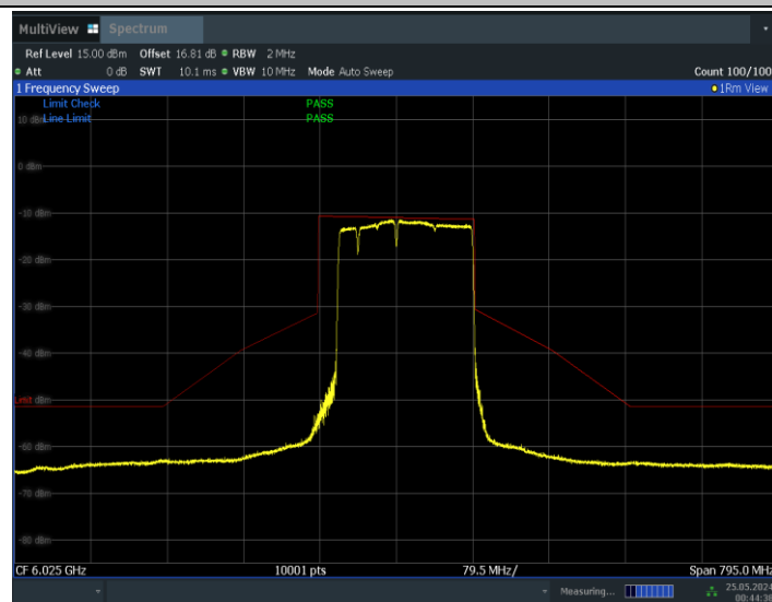
11BE160MIMO_Ant1_6025_996+484+242_Non-OFDMA_1
