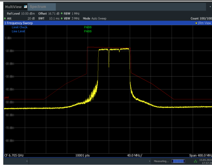
11BE80MIMO_Ant0_6705_484+242_Non-OFDMA_1
