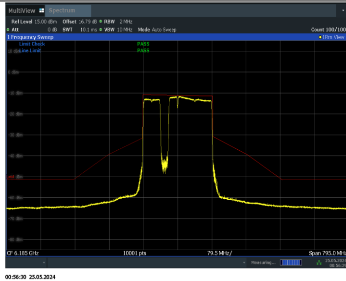
11BE160MIMO_Ant1_6185_996+484+242_Non-OFDMA_4
