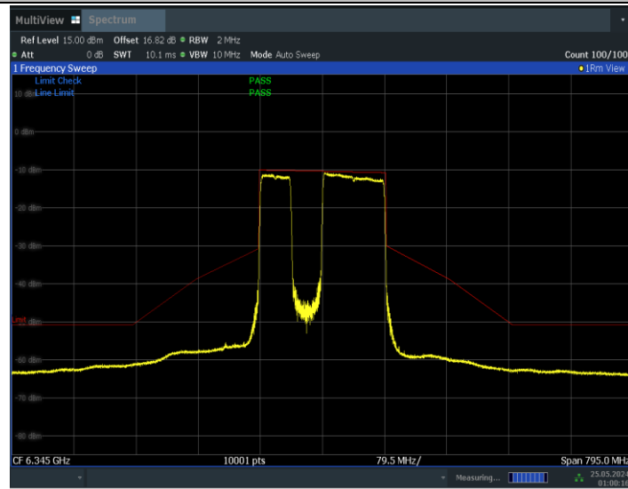
11BE160MIMO_Ant0_6345_996+484_Non-OFDMA_3
