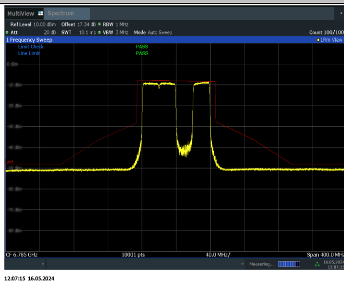
11BE80MIMO_Ant1_6785_484+242_Non-OFDMA_3
