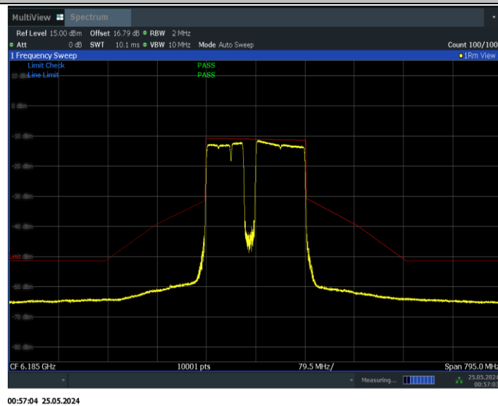
11BE160MIMO_Ant1_6185_996+484+242_Non-OFDMA_5
