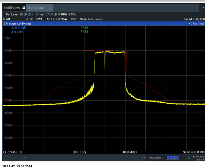
11BE80MIMO_Ant1_6945_484+242_Non-OFDMA_2
