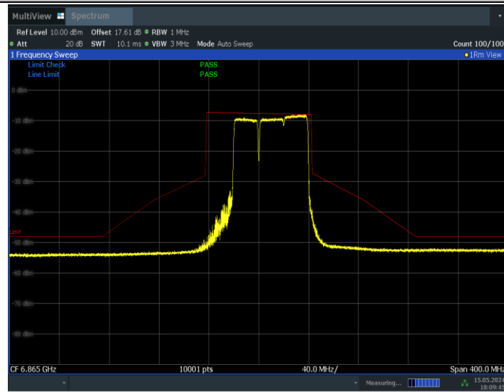
11BE80MIMO_Ant1_6865_484+242_Non-OFDMA_1
