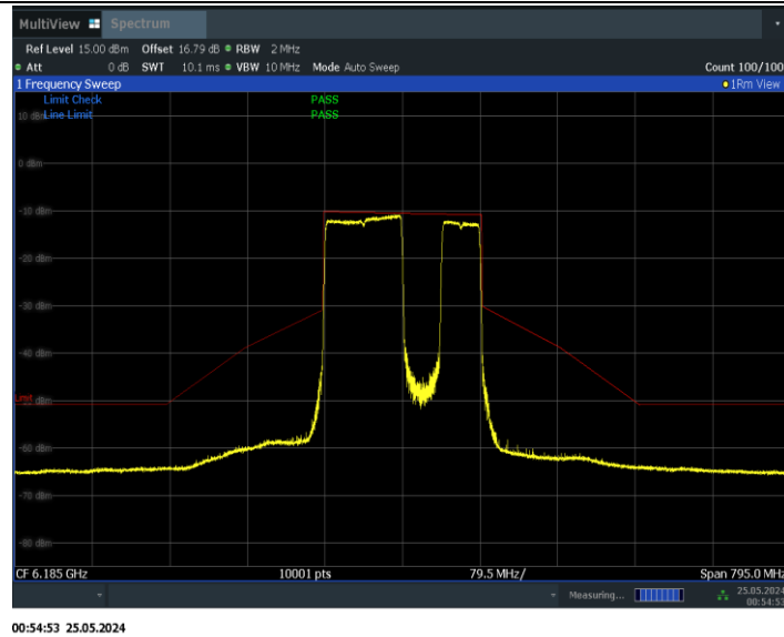
11BE160MIMO_Ant1_6185_996+484_Non-OFDMA_3
