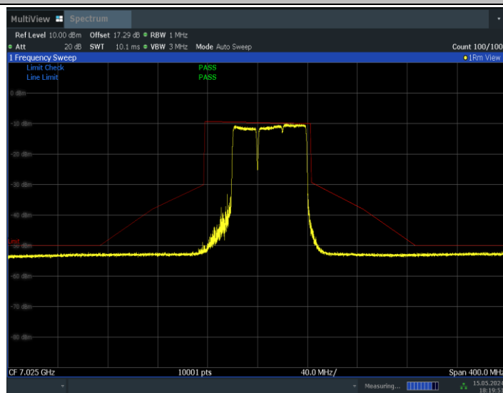
11BE80MIMO_Ant1_7025_484+242_Non-OFDMA_1
