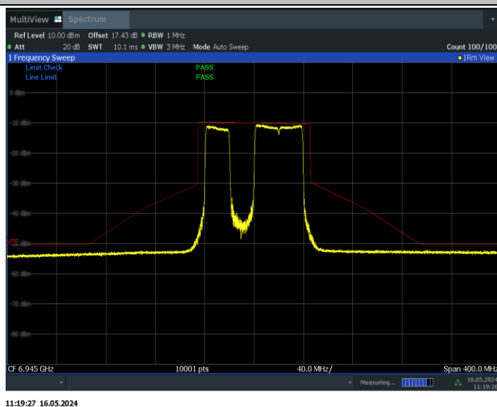
11BE80MIMO_Ant1_6945_484+242_Non-OFDMA_2
