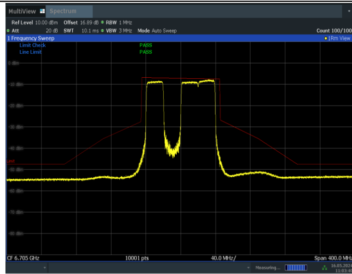
11BE80MIMO_Ant1_6705_484+242_Non-OFDMA_2
