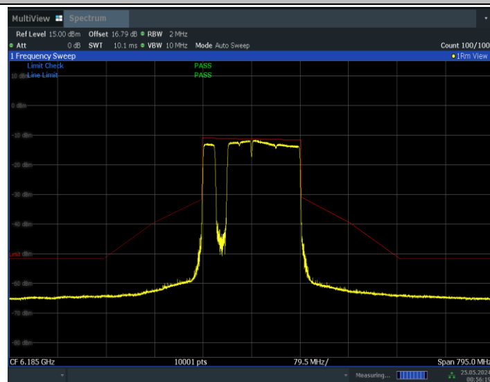
11BE160MIMO_Ant1_6185_996+484+242_Non-OFDMA_2
