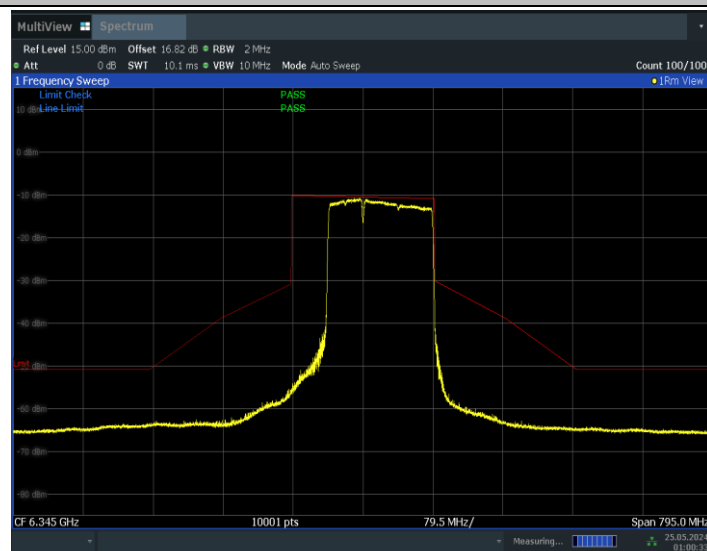
11BE160MIMO_Ant0_6345_996+484_Non-OFDMA_4
