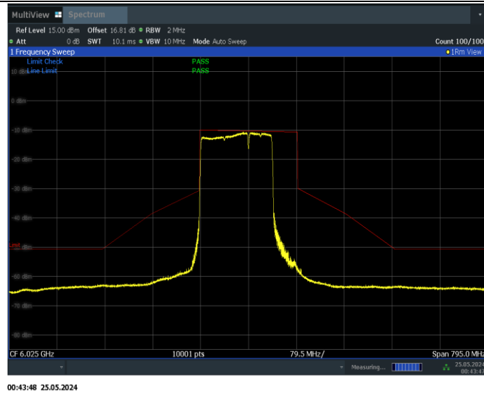
11BE160MIMO_Ant1_6025_996+484_Non-OFDMA_2
