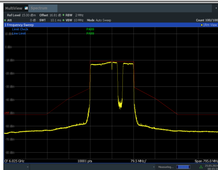
11BE160MIMO_Ant1_6025_996+484+242_Non-OFDMA_6
