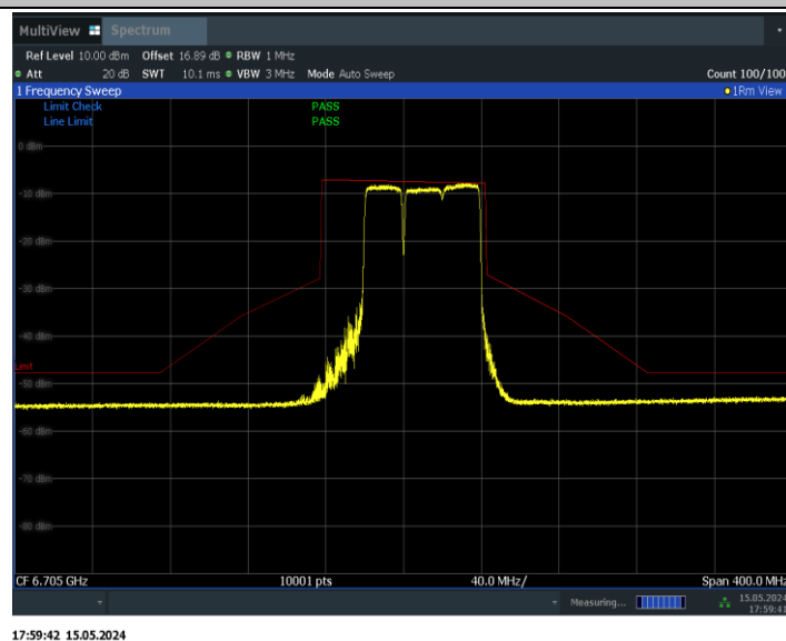
11BE80MIMO_Ant1_6705_484+242_Non-OFDMA_1
