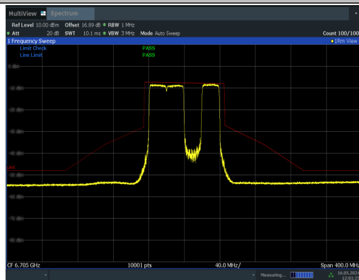
11BE80MIMO_Ant1_6705_484+242_Non-OFDMA_3
