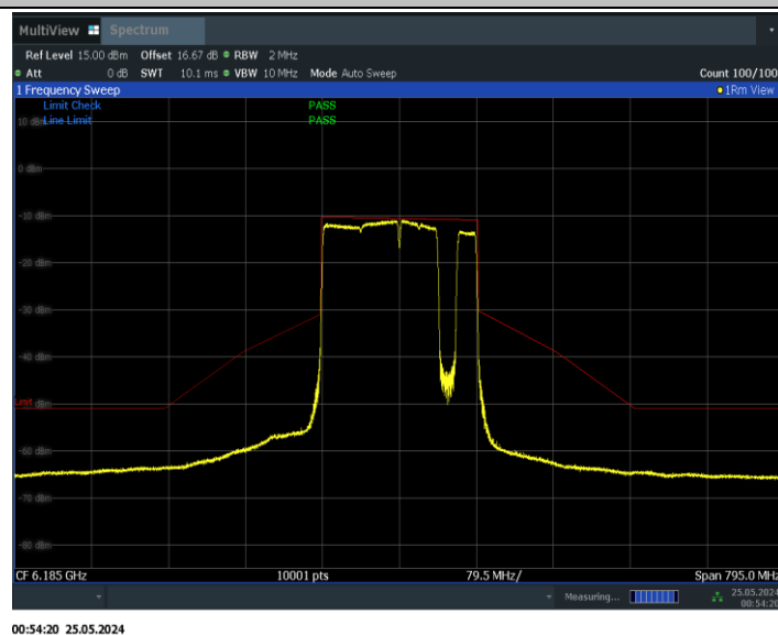
11BE160MIMO_Ant0_6185_996+484+242_Non-OFDMA_7
