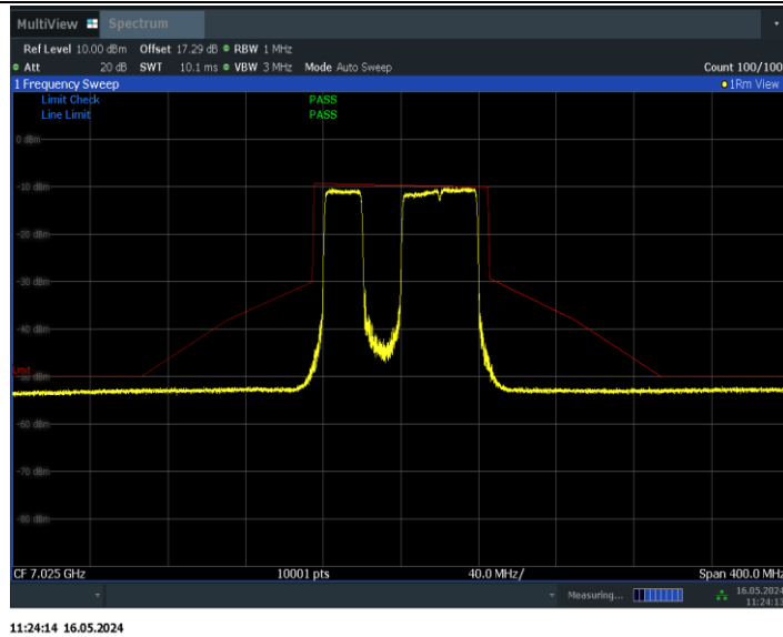
11BE80MIMO_Ant1_7025_484+242_Non-OFDMA_3
