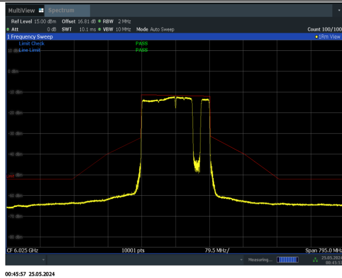
11BE160MIMO_Ant1_6025_996+484+242_Non-OFDMA_8
