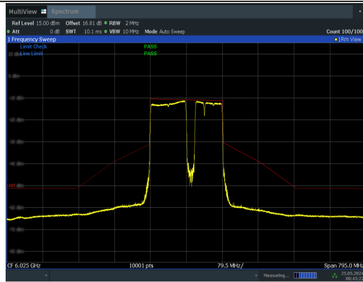
11BE160MIMO_Ant1_6025_996+484+242_Non-OFDMA_5
