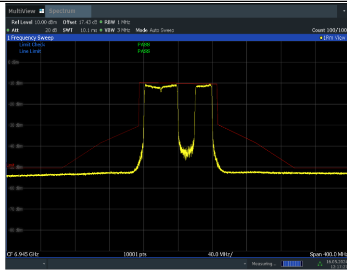
11BE80MIMO_Ant1_6945_484+242_Non-OFDMA_3
