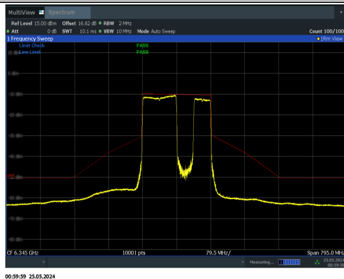
11BE160MIMO_Ant0_6345_996+484_Non-OFDMA_2
