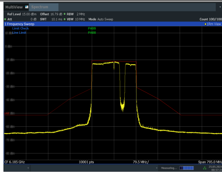
11BE160MIMO_Ant1_6185_996+484+242_Non-OFDMA_6
