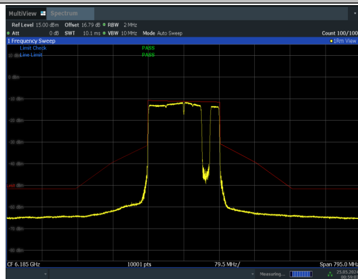
11BE160MIMO_Ant1_6185_996+484+242_Non-OFDMA_7
