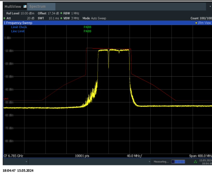
11BE80MIMO_Ant1_6785_484+242_Non-OFDMA_2
