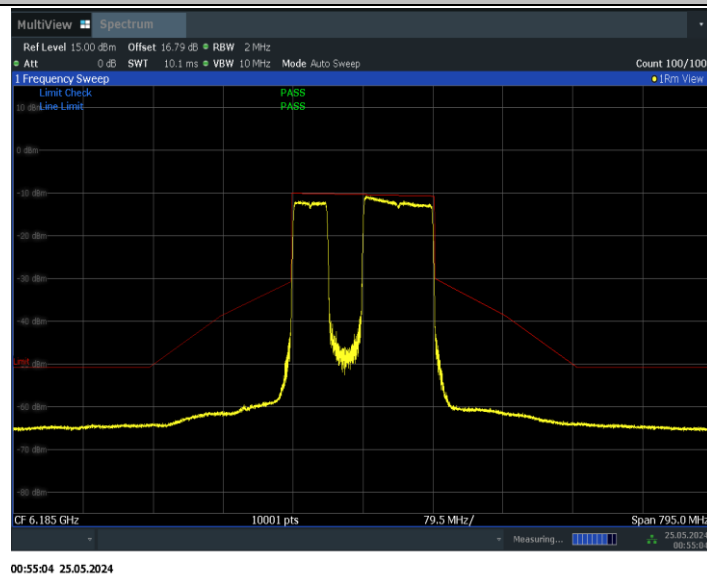
11BE160MIMO_Ant1_6185_996+484_Non-OFDMA_4
