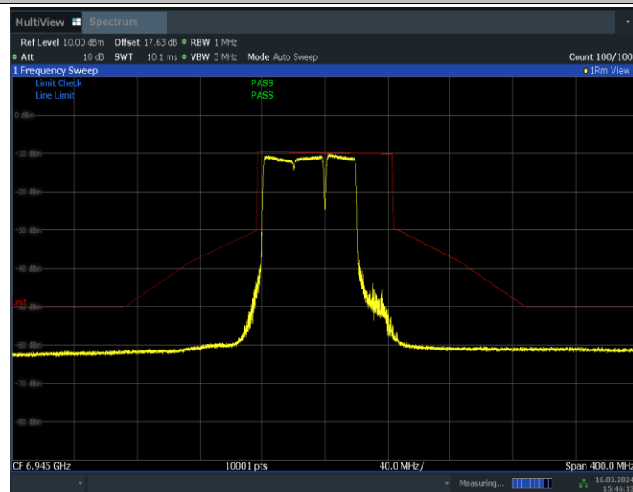
11BE80MIMO_Ant1_6945_484+242_Non-OFDMA_4
