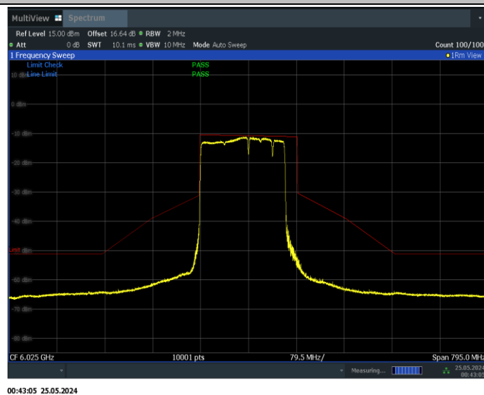
11BE160MIMO_Ant1_6025_996+484_Non-OFDMA_1
