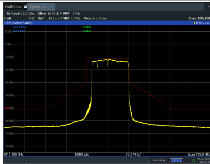
11BE160MIMO_Ant1_6185_996+484+242_Non-OFDMA_1
