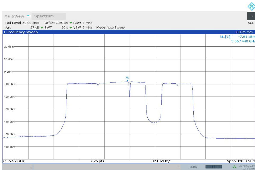
11BE160MIMO_Ant1_5570_996+484+242_OFDMA_7
