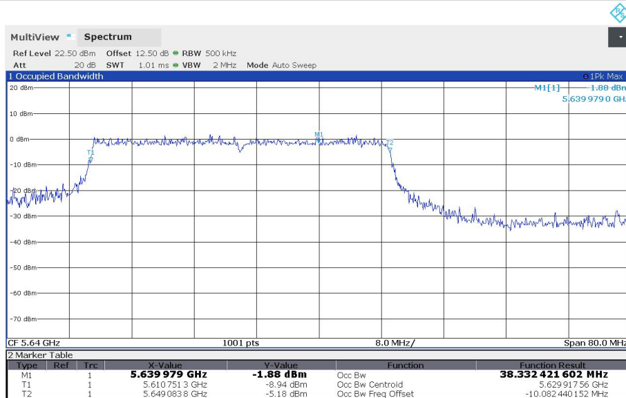
11BE160MIMO_Ant1_5570_Puncturing 20M_7
