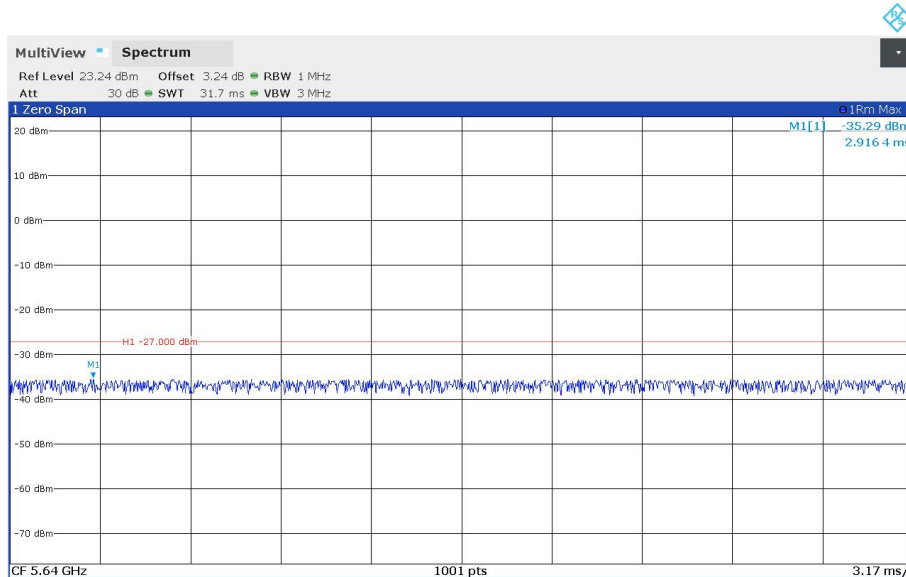
11BE160MIMO_Ant1_5570_Puncturing20- configure-8
