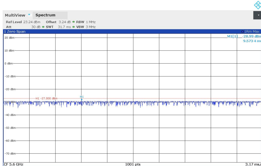
11BE160MIMO_Ant1_5570_Puncturing20- configure-6
