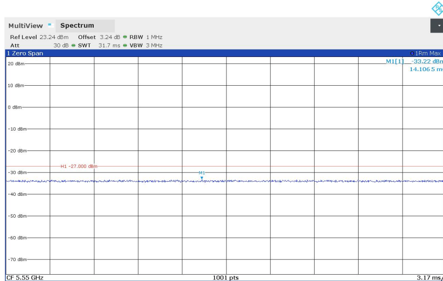
11BE160MIMO_Ant1_5570_Puncturing40- configure-2
