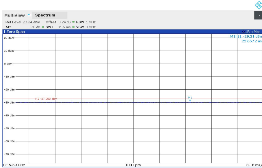
11BE160MIMO_Ant1_5570_Puncturing40- configure-4
