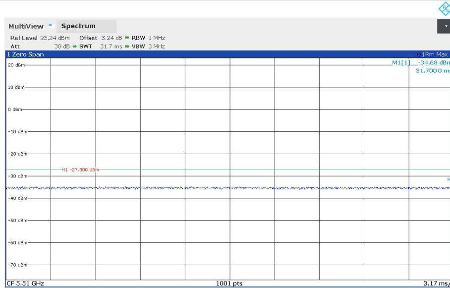
11BE160MIMO_Ant1_5570_Puncturing40- configure-2
