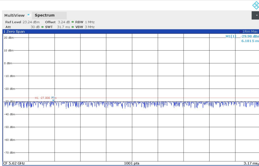
11BE160MIMO_Ant1_5570_Puncturing20- configure-8
