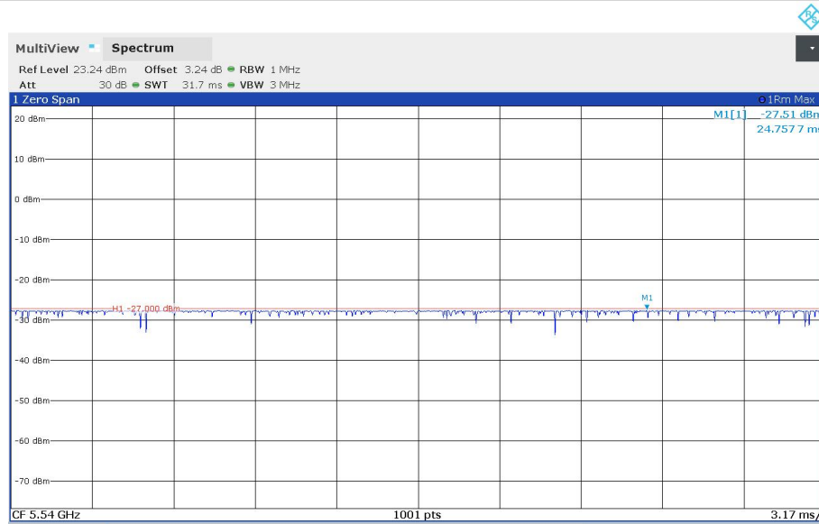
11BE160MIMO_Ant1_5570_Puncturing20- configure-4
