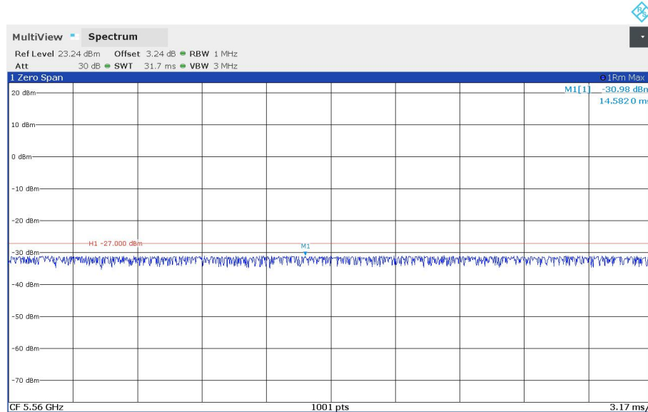
11BE160MIMO_Ant1_5570_Puncturing20- configure-4
