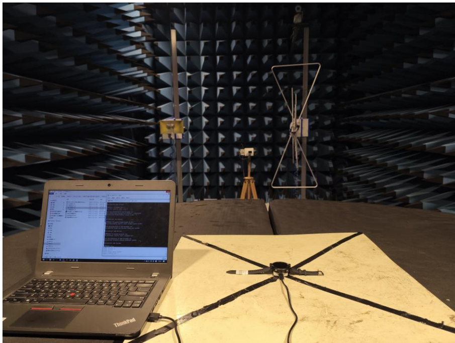
Radiated Emission Above 18 GHz -26.5 GHz
