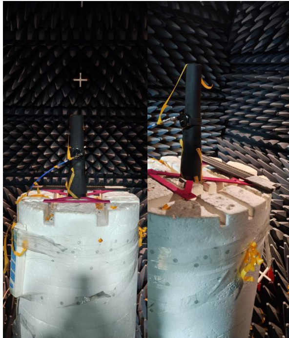
Fig.5. The DUT in the fully anechoic chamber
