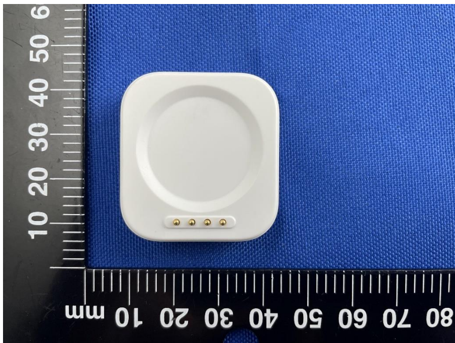
Accessory-Charging Base
