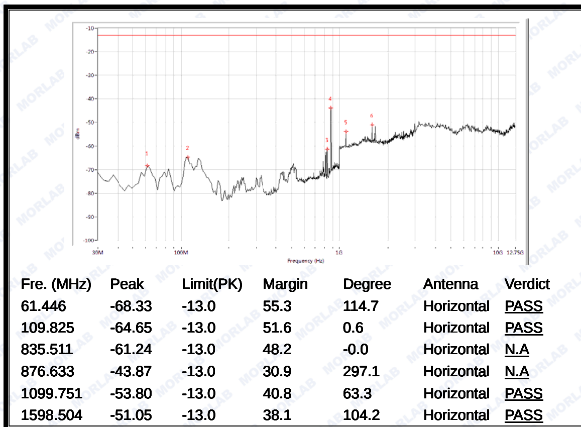
(Plot E.3: WCDMA 850MHz Channel = 4175, Test Antenna Horizontal)
