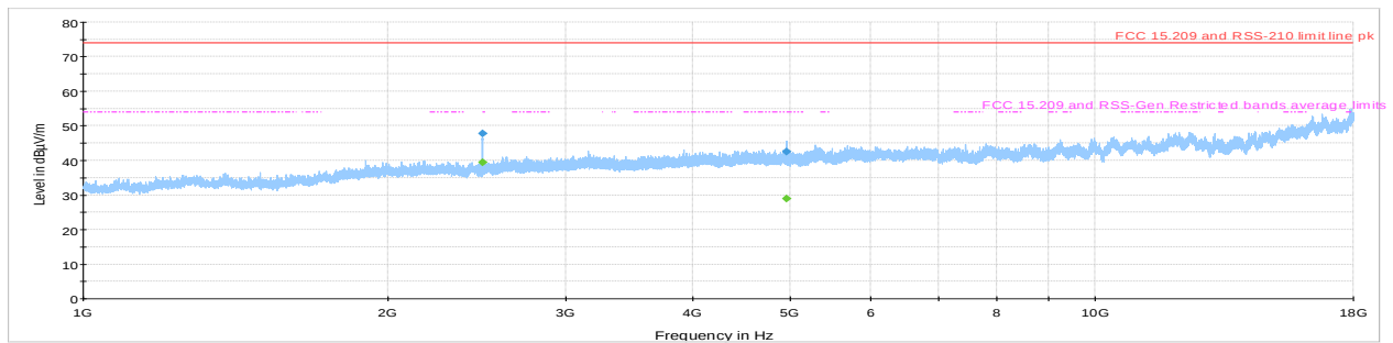
Figure 8.6-9: Radiated Spurious emissions 1 - 18GHz, mid channel
