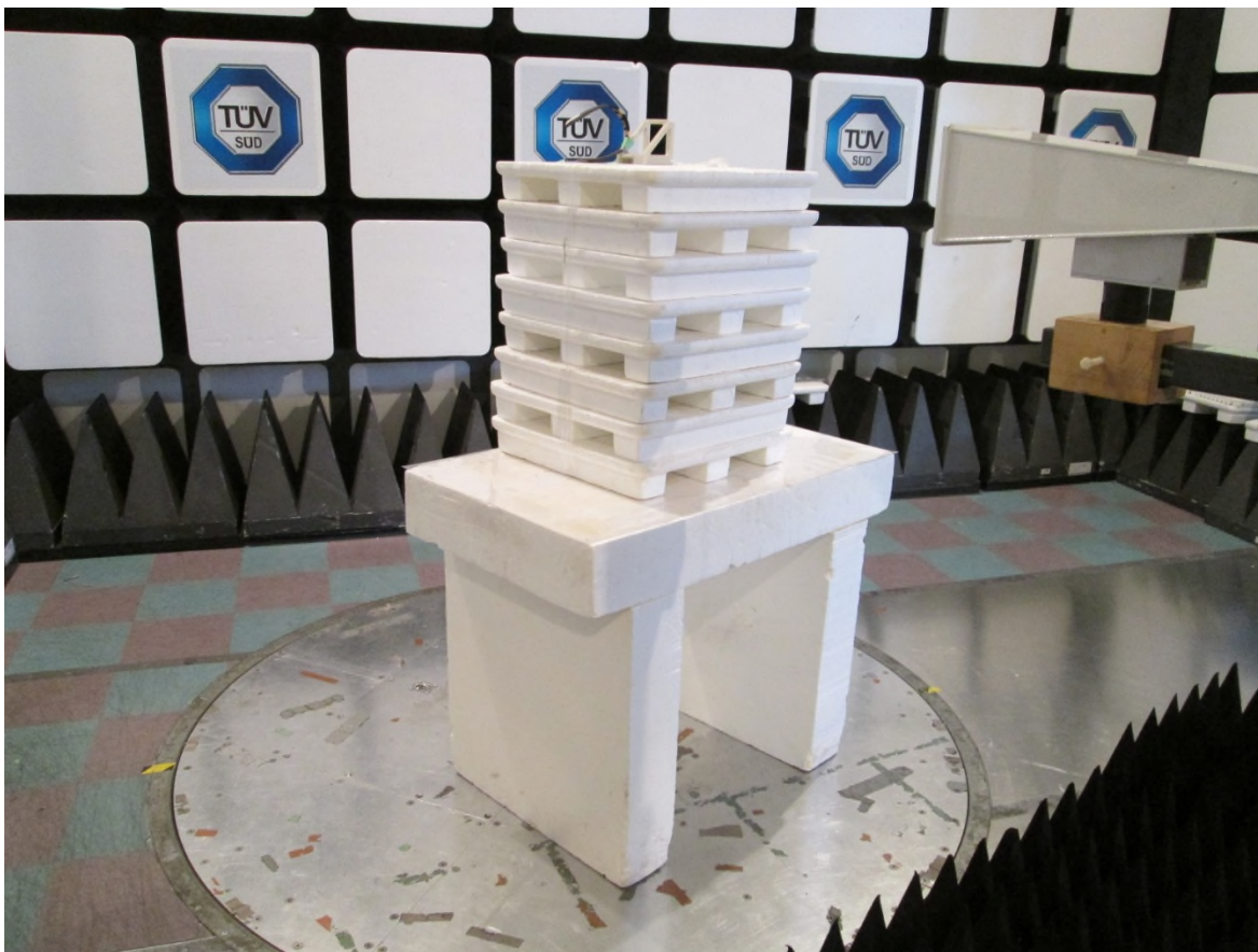
Test setup photo 5 Radiated measurements, 10 GHz – 18 GHz
