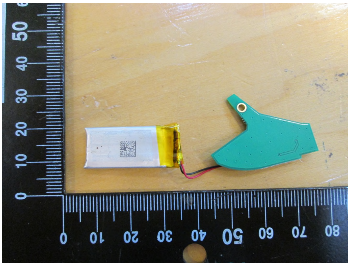
EUT – Internal view 9 Left side PCB, side 2
