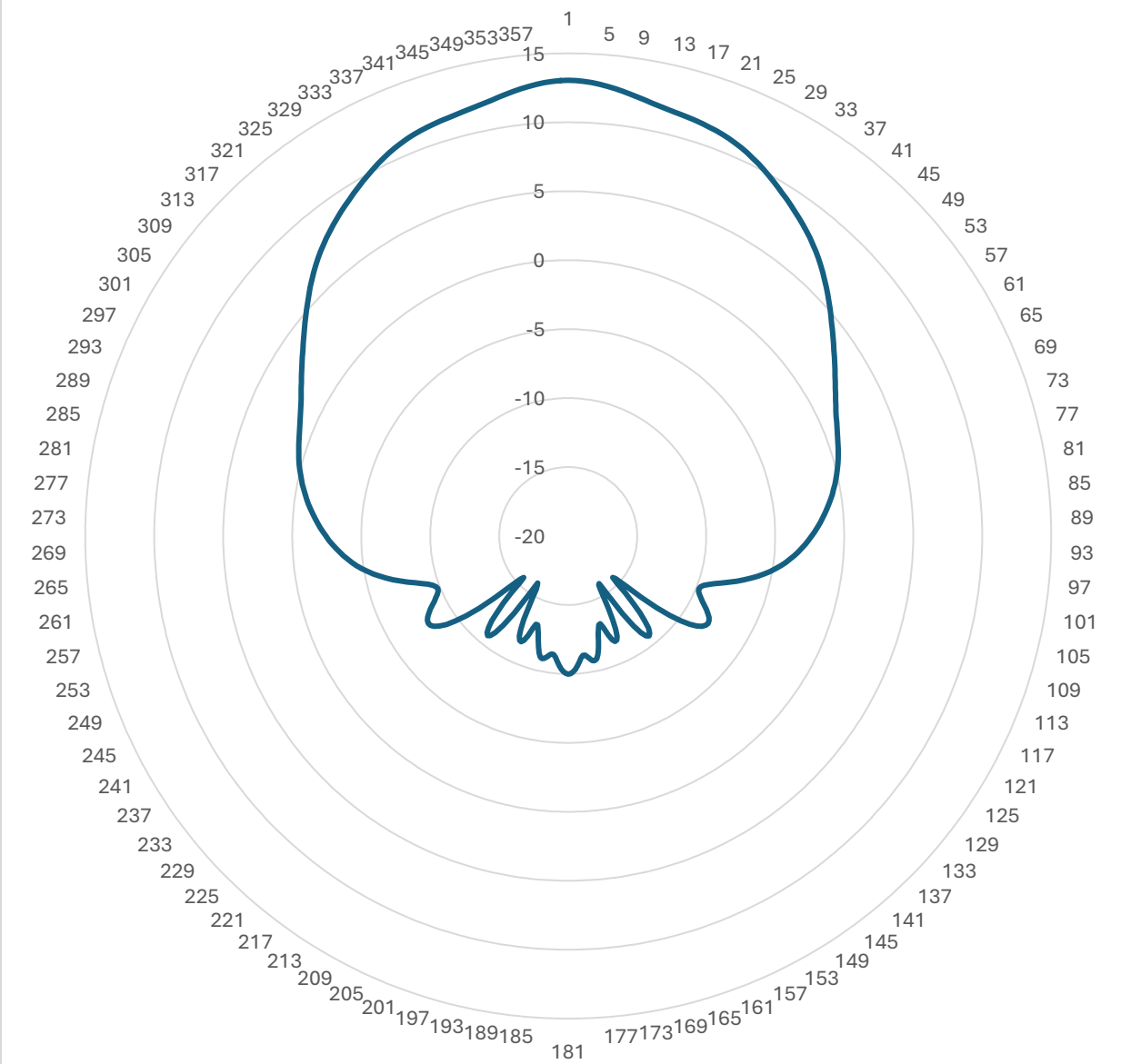
5.3GHz, C6 Azimuth Plane Gain (dBi), Peak Gain = 13dBi
