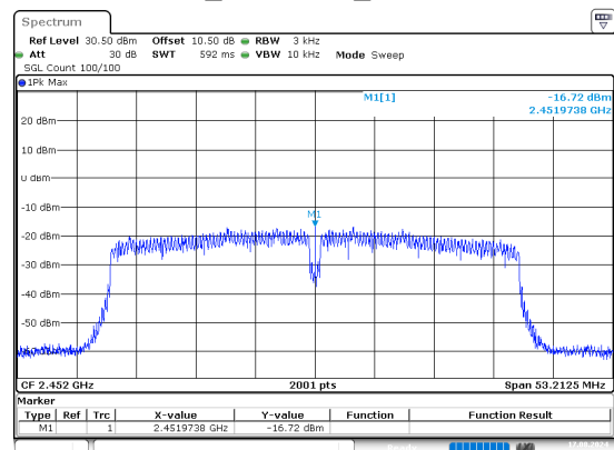
n40_2452MHz_Chain 1
