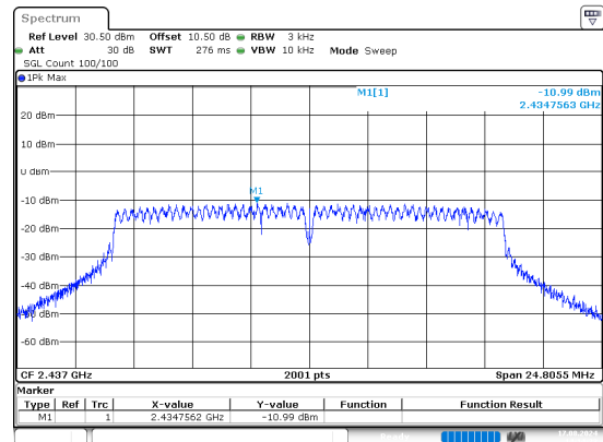
g_2437MHz_Chain 1
