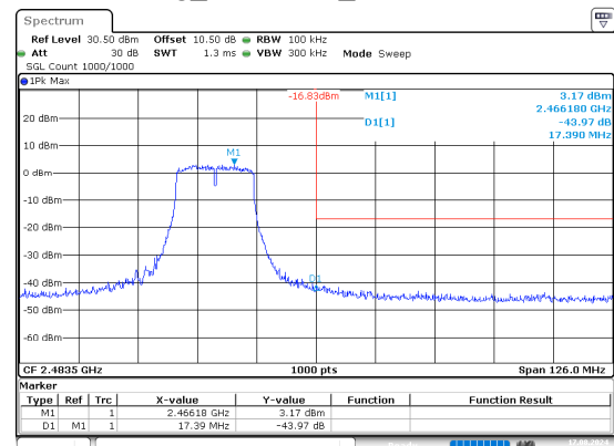
g_2462MHz_Chain 1
