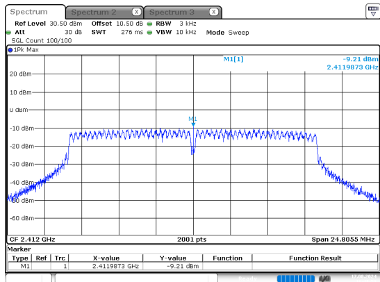
g_2412MHz_Chain 0
