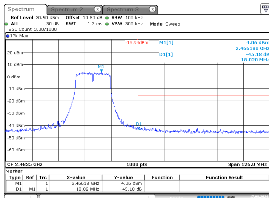
g_2462MHz_Chain 0
