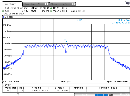
g_2437MHz_Chain 0
