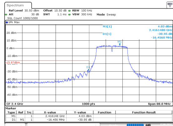
g_2412MHz_Chain 1
