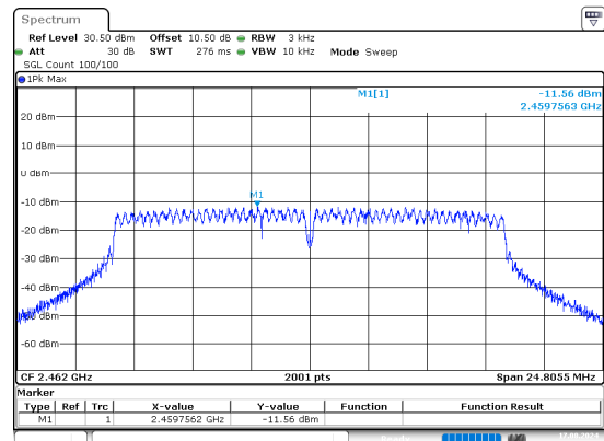
g_2462MHz_Chain 1
