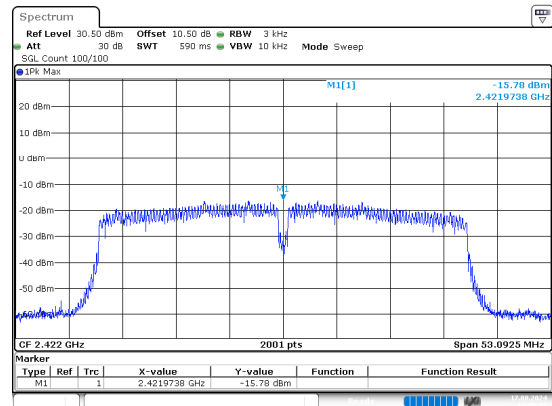
n40_2422MHz_Chain 1
