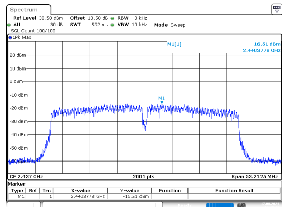
n40_2437MHz_Chain 1
