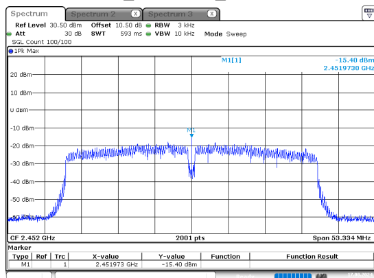
n40_2452MHz_Chain 0
