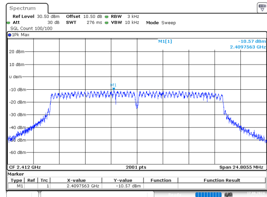
g_2412MHz_Chain 1
