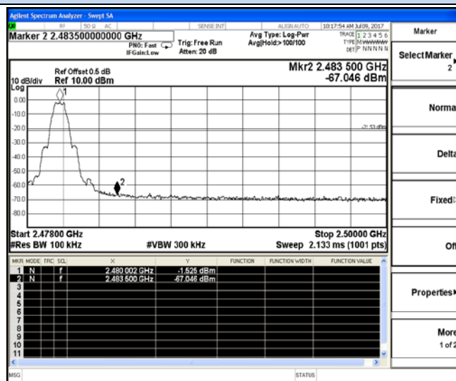
Channel 39 / 2480 MHz
