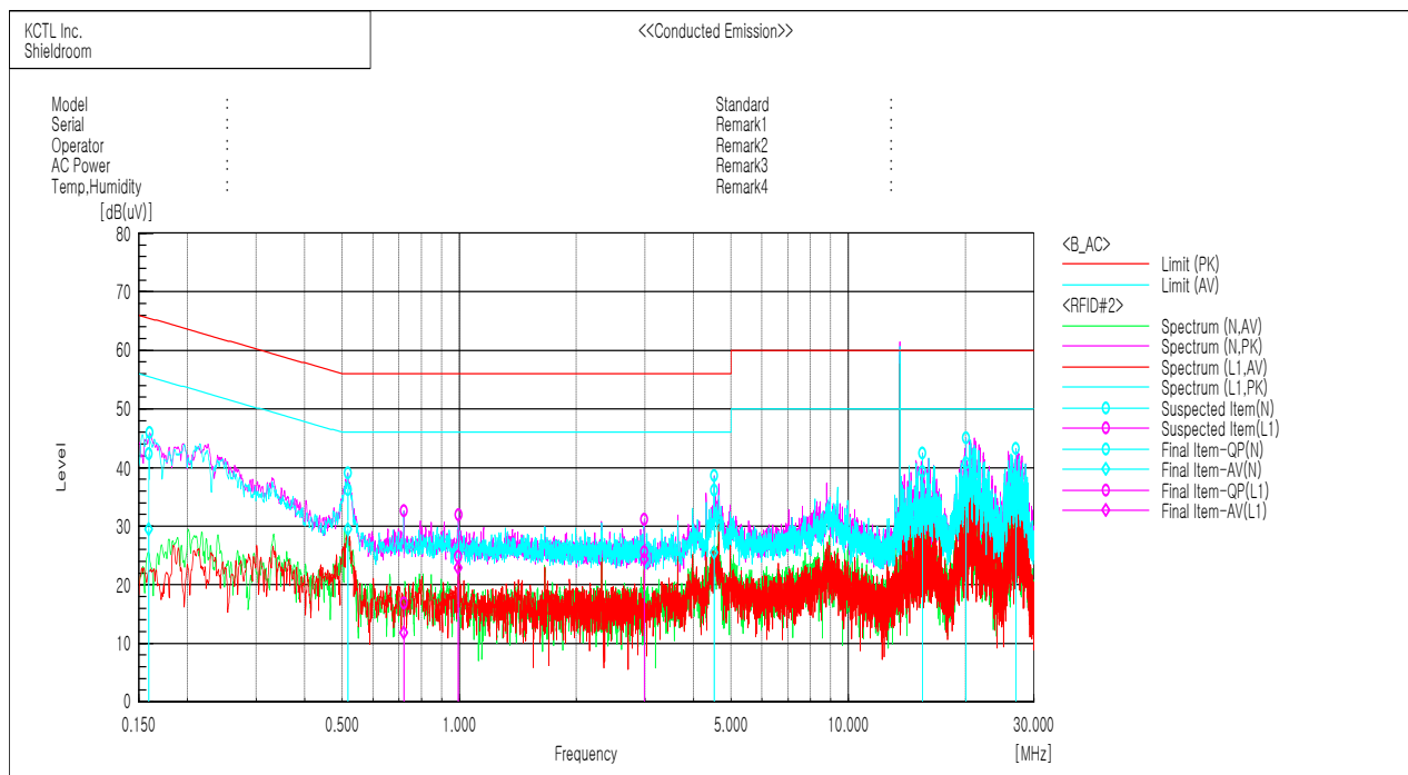
Figure4. The plot of Conducted Emission
