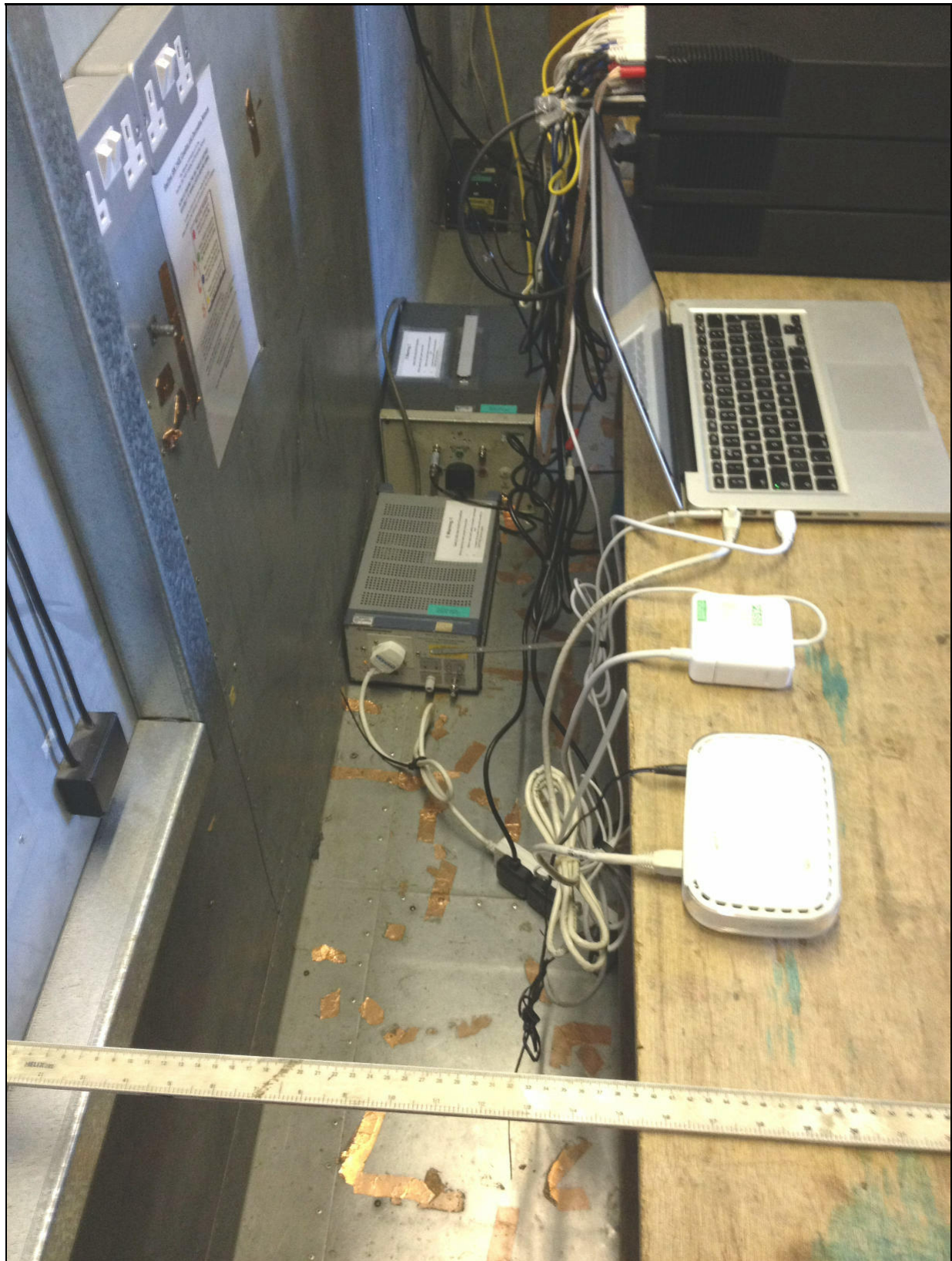
Photograph 5 Conducted Emissions - 8dac - USB Source
