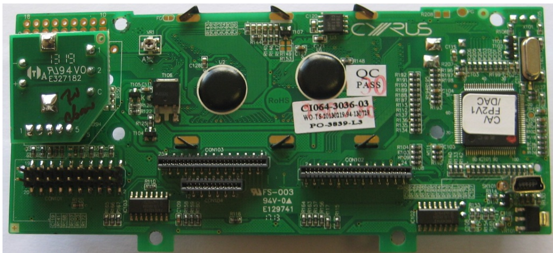
8. Display PCB rear view: Cyrus PRE DAC
