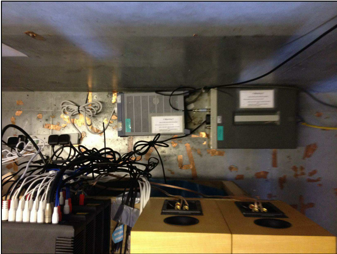
Photograph 4 Radiated Emissions
