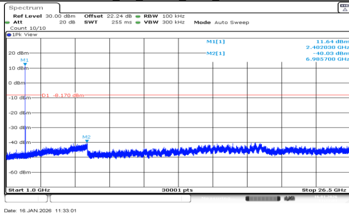
BLE_2M_Ant_BT_2402_1000~26500
