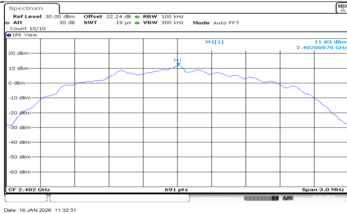
BLE_2M_Ant_BT_2402_0~Reference
