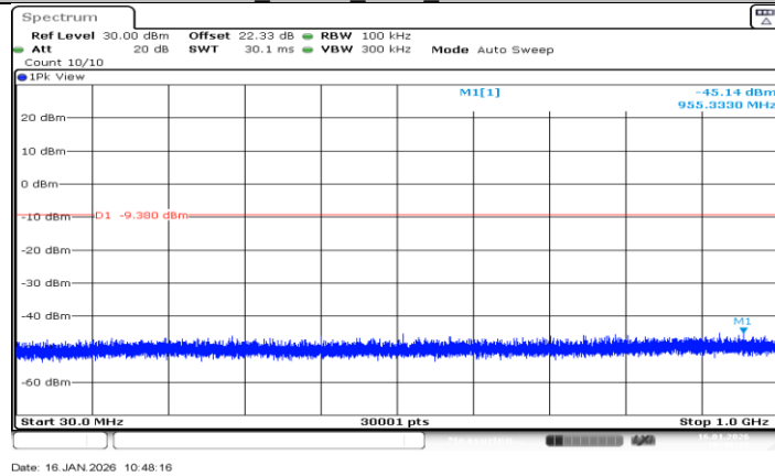
DH5 Ant BT 2441_30~1000
