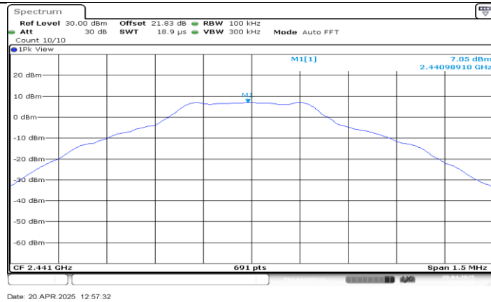
DH5_Ant BT_2441_0~Reference
