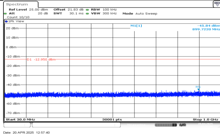
DH5_Ant BT_2441_30~1000
