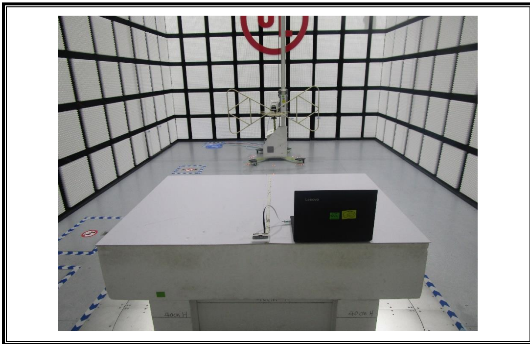
RADIATED RF MEASUREMENT SETUP (Below 1 GHz)
