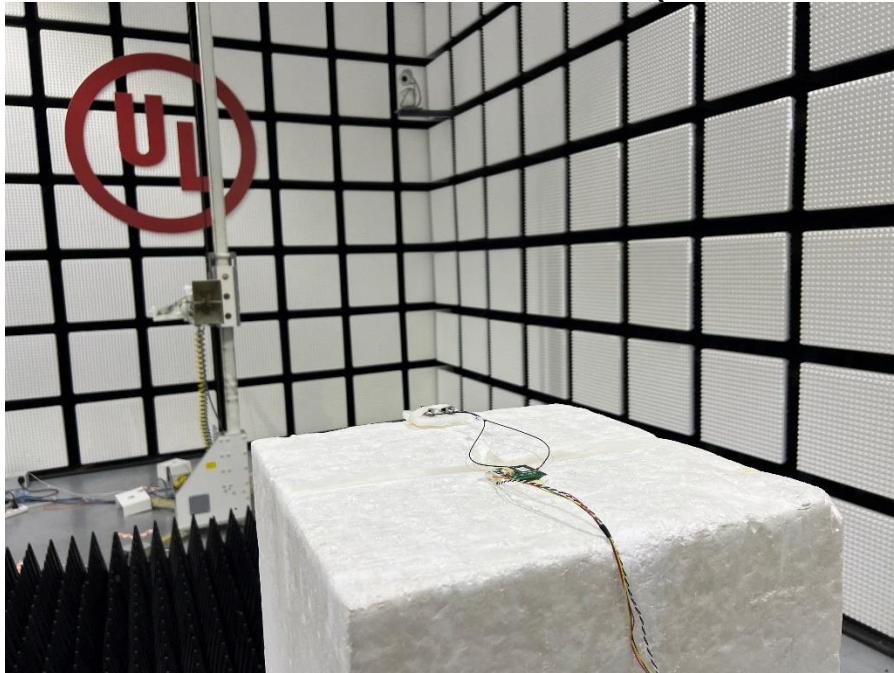
RADIATED RF MEASUREMENT SETUP (Above 1G
