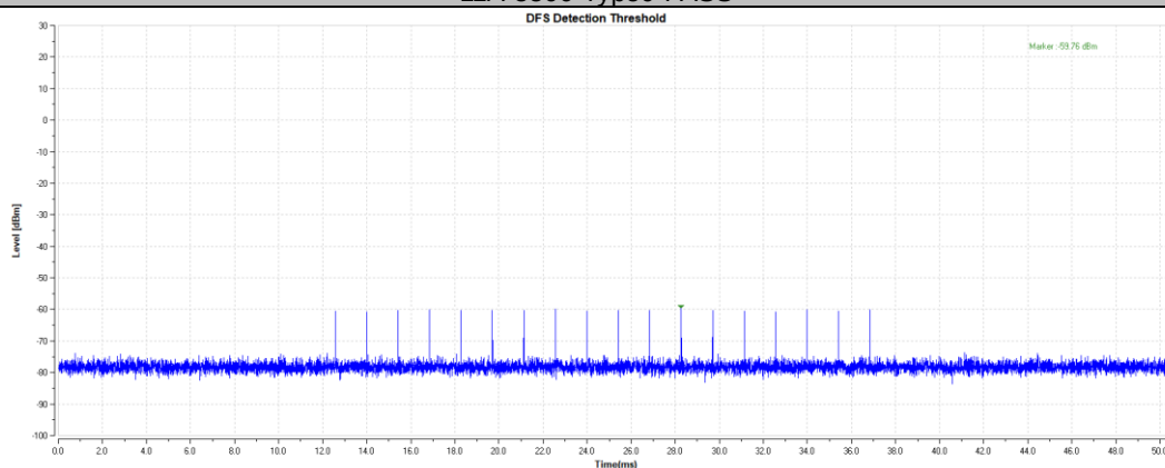
11N40SISO-5270-Type0-PASS
