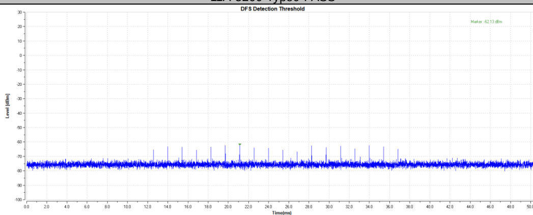
11A-5500-Type0-PASS
