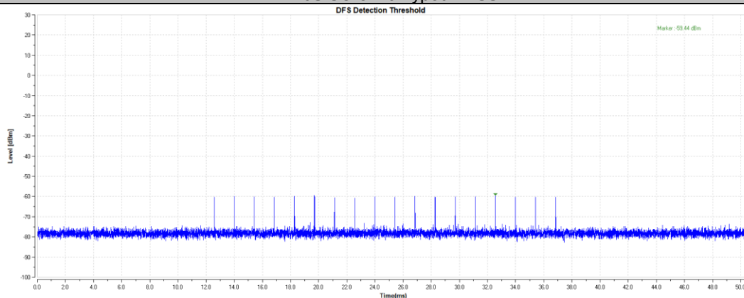
11N40SISO-5510-Type0-PASS
