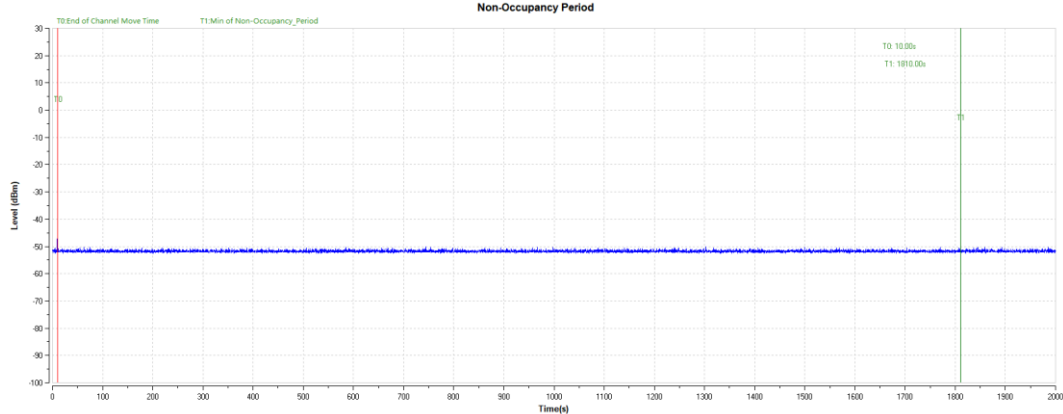
11A-5500-Type0-PASS
