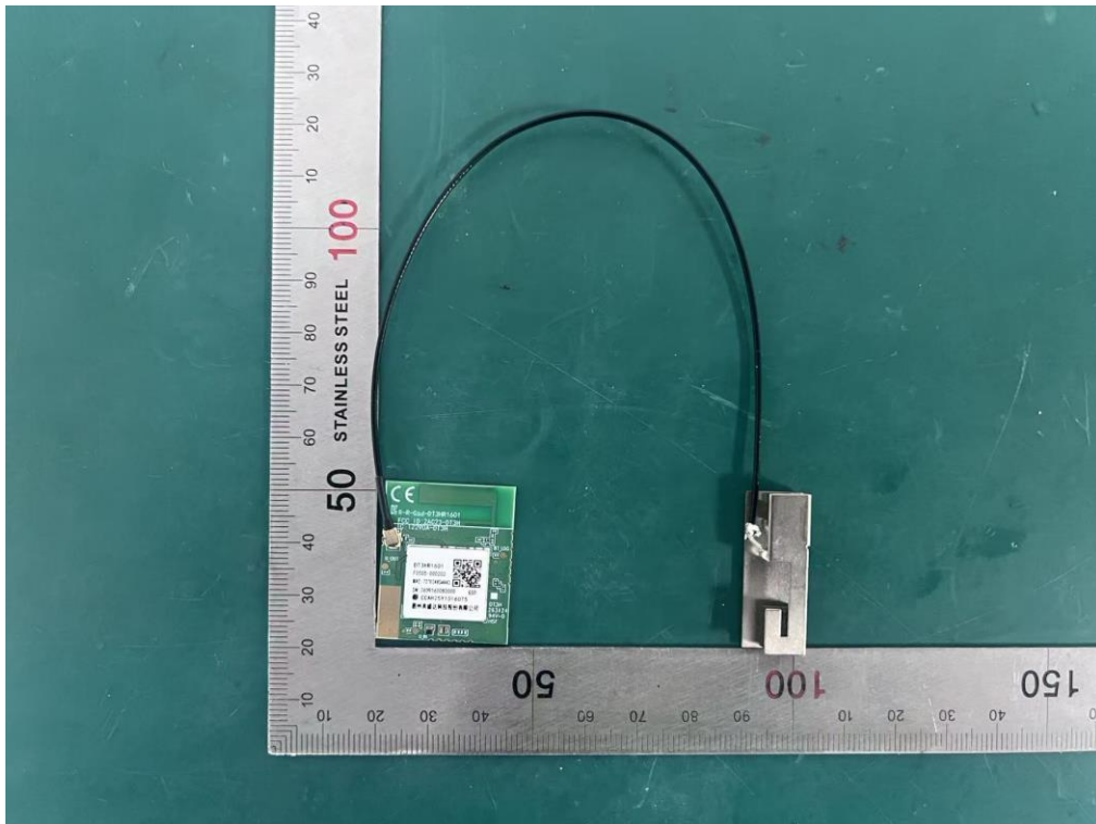
External Photos M/N: DT3HR1601
