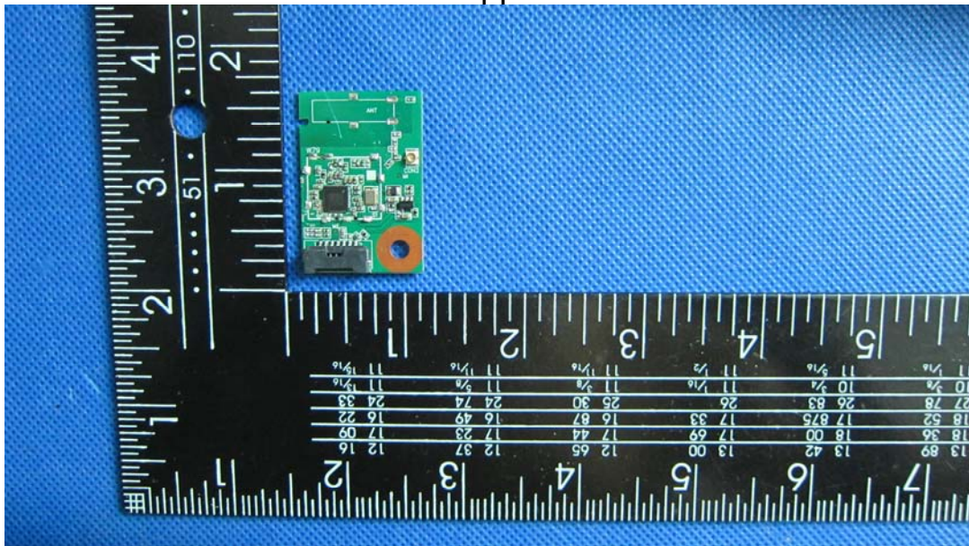
Photo 5 Appearance of PCB
