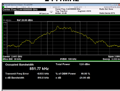
2441MHz
