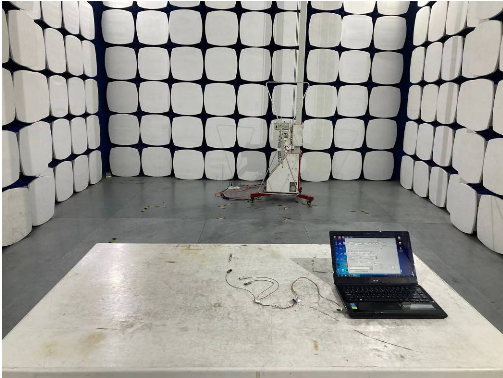
Test Setup Below 1GHz
