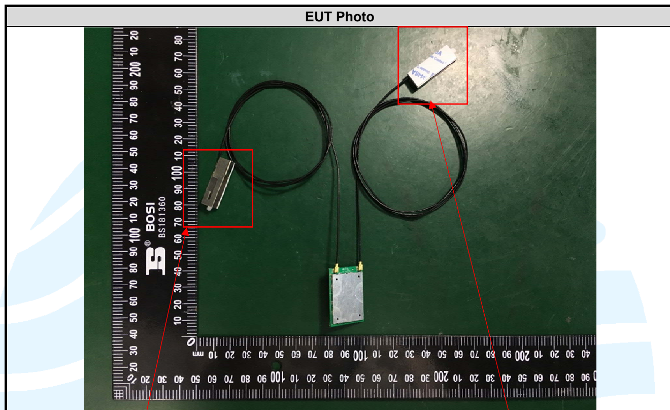
Antenna 1 (WI-FI)
