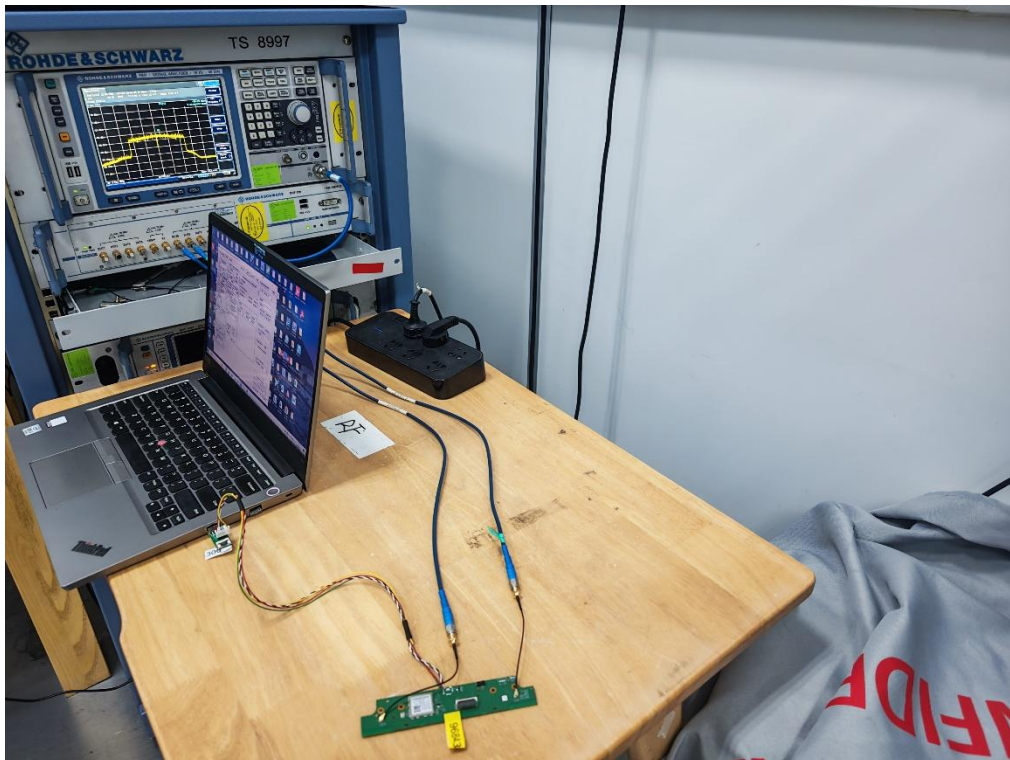
RF CONDUCTION MEASUREMENT SETUP
