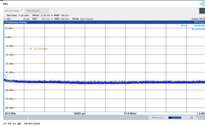
BLE_1M_Ant1_2480_30~1000
