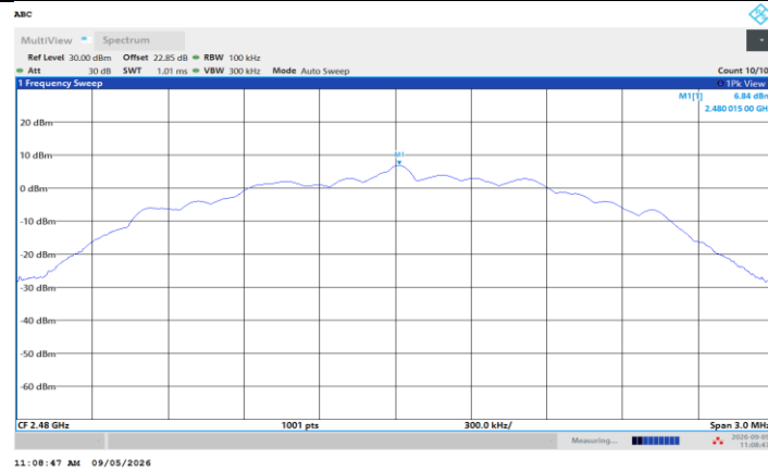
BLE_2M_Ant1_2480_0~Reference
