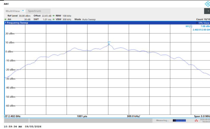
BLE_2M_Ant1_2402_0~Reference
