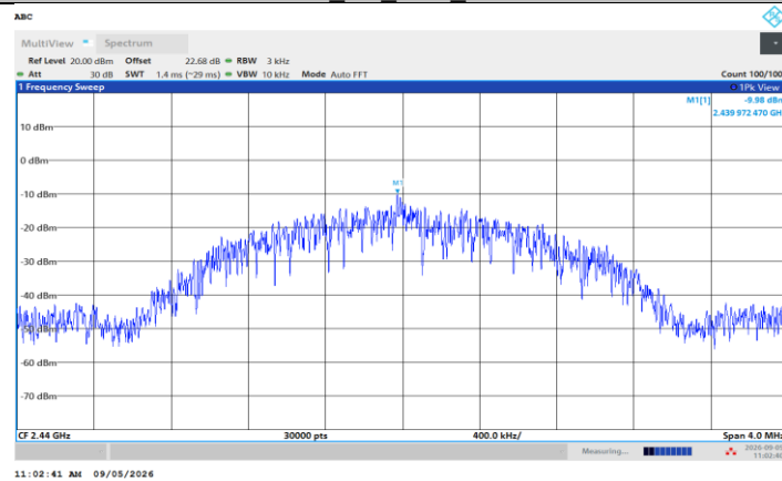
BLE_2M_Ant1_2440
