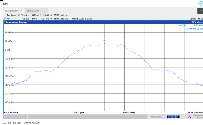
BLE_1M_Ant1_2480_0~Reference
