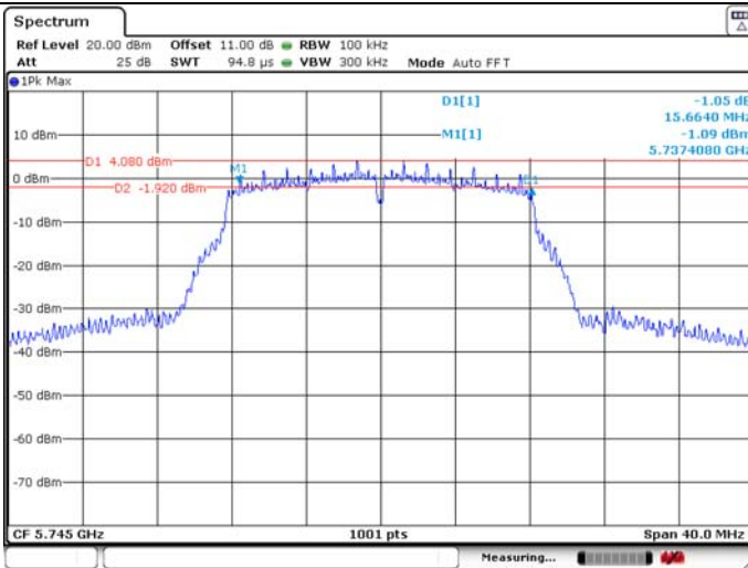
6dB Bandwidth
