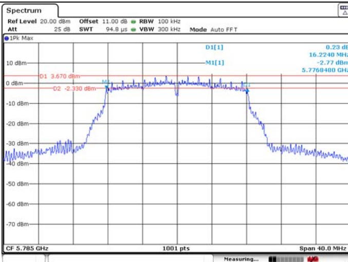
6dB Bandwidth
