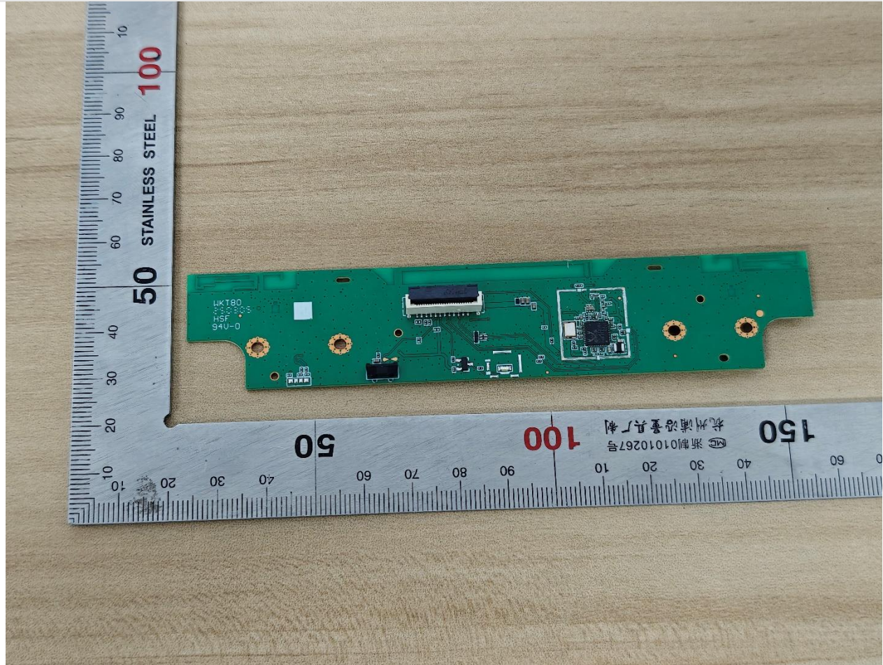
Internal View of EUT-1
