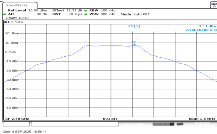
DH5_Ant3_2480_0~Reference
