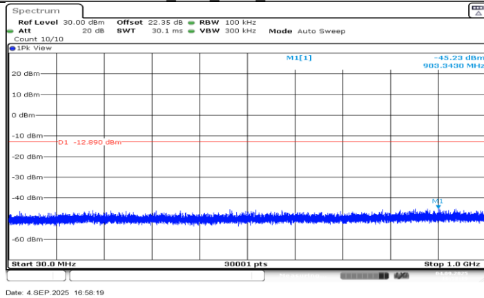
DH5_Ant3_2480_30~1000
