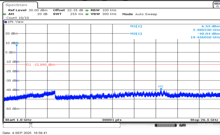
DH5_Ant3_2480_1000~26500
