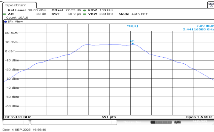
DH5_Ant3_2441_0~Reference
