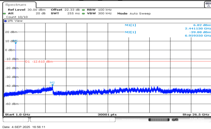
DH5_Ant3_2441_1000~26500
