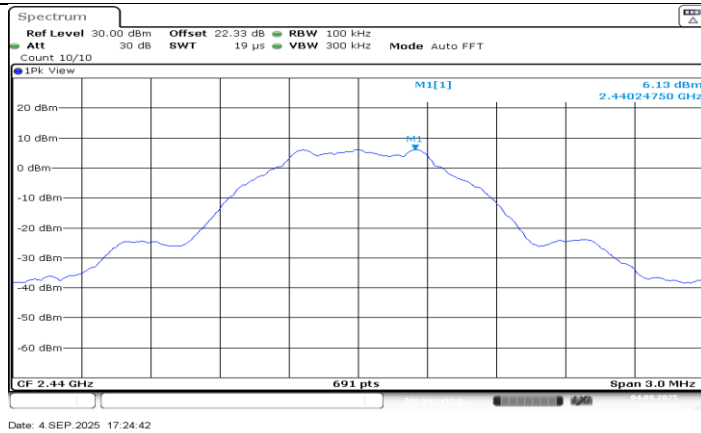
BLE_1M_Ant3_2440_0~Reference
