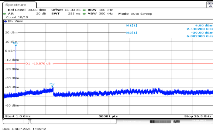
BLE_1M_Ant3_2440_1000~26500
