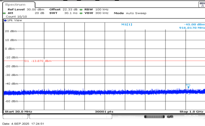
BLE_1M_Ant3_2440_30~1000
