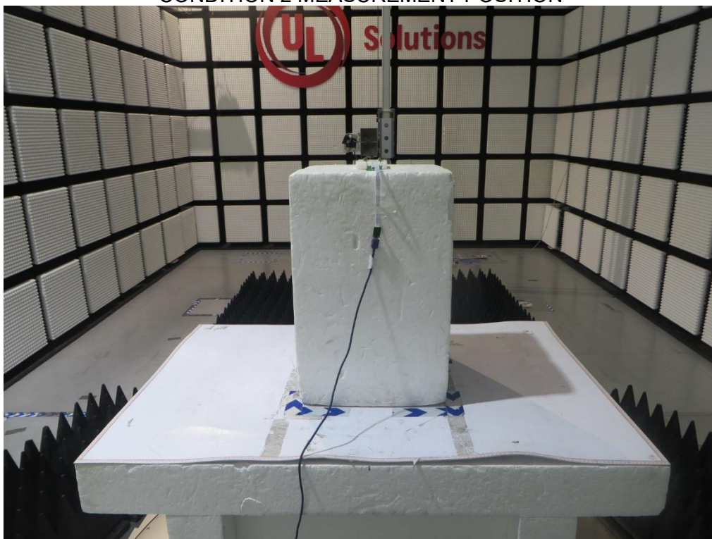
CONDITION 2 MEASUREMENT POSITION (X axis)
