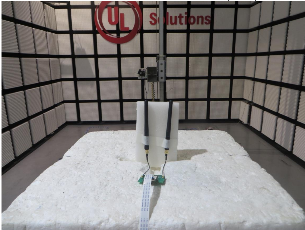
CONDITION 2 MEASUREMENT POSITION (Z axis)
