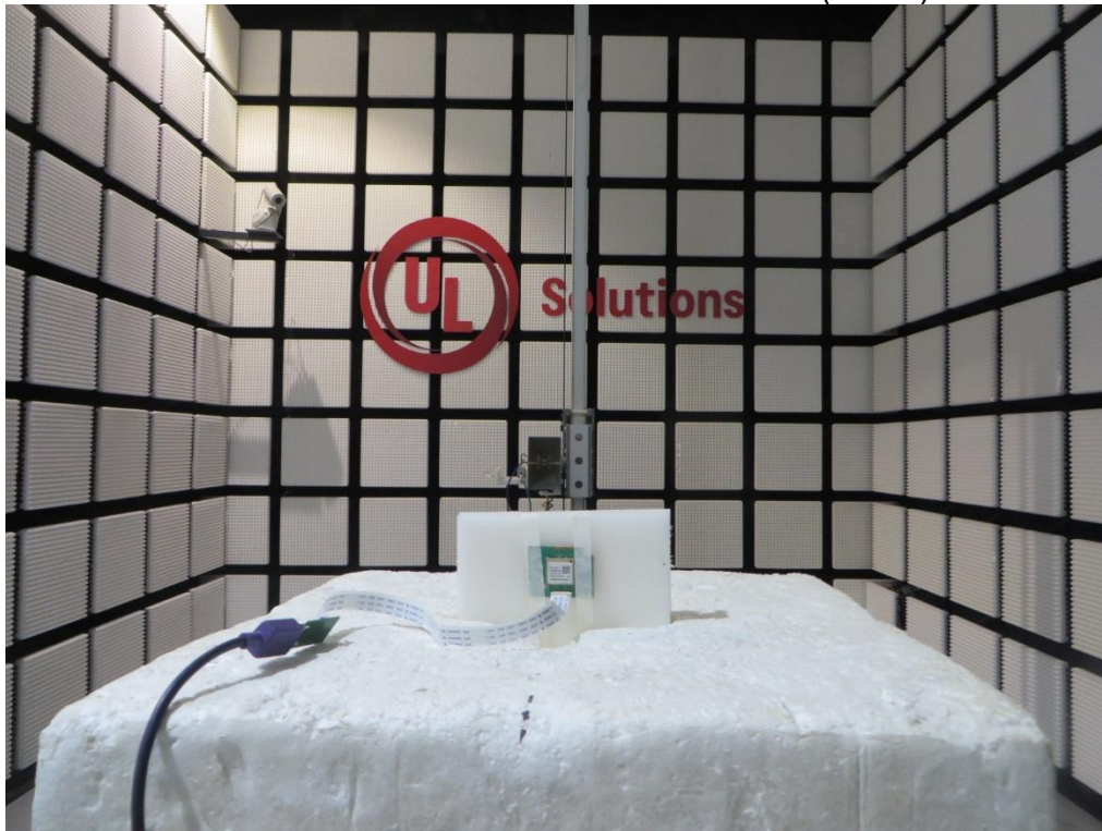
CONDITION 1 MEASUREMENT POSITION (Z axis)
