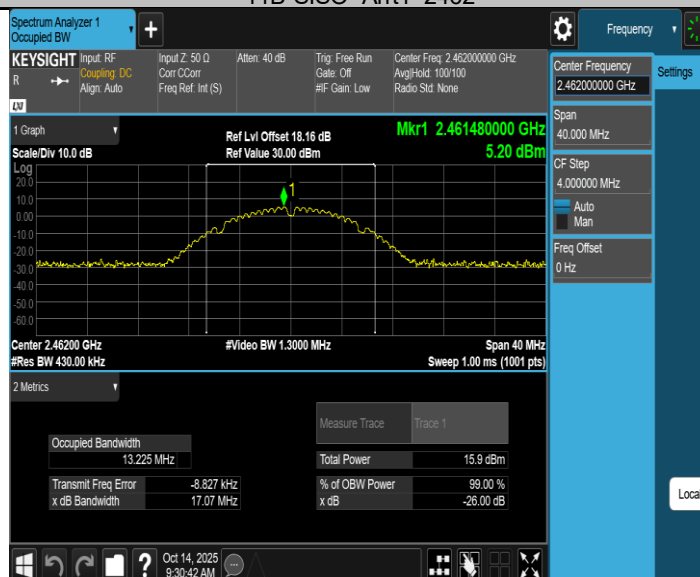
11B-SISO Ant2 2462
