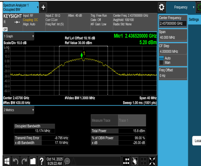
11B-SISO Ant2 2437
