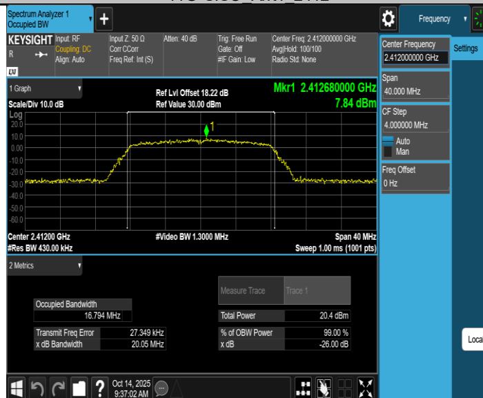
11G-SISO Ant2 2412
