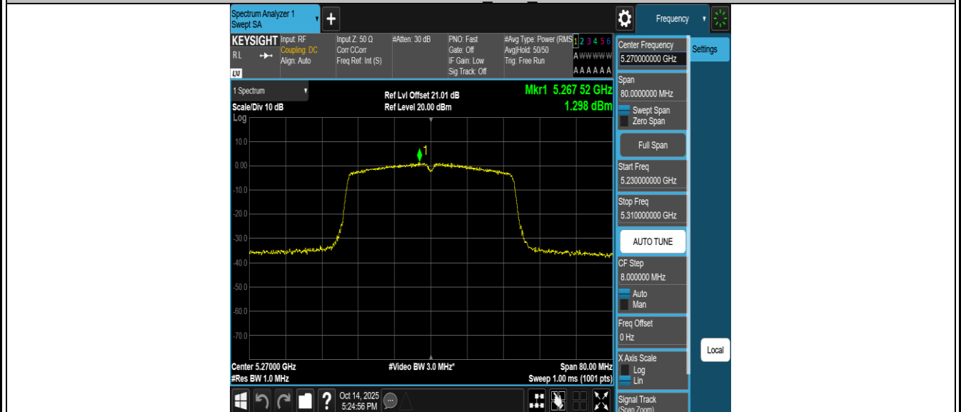
11N40MIMO Ant2 5270
