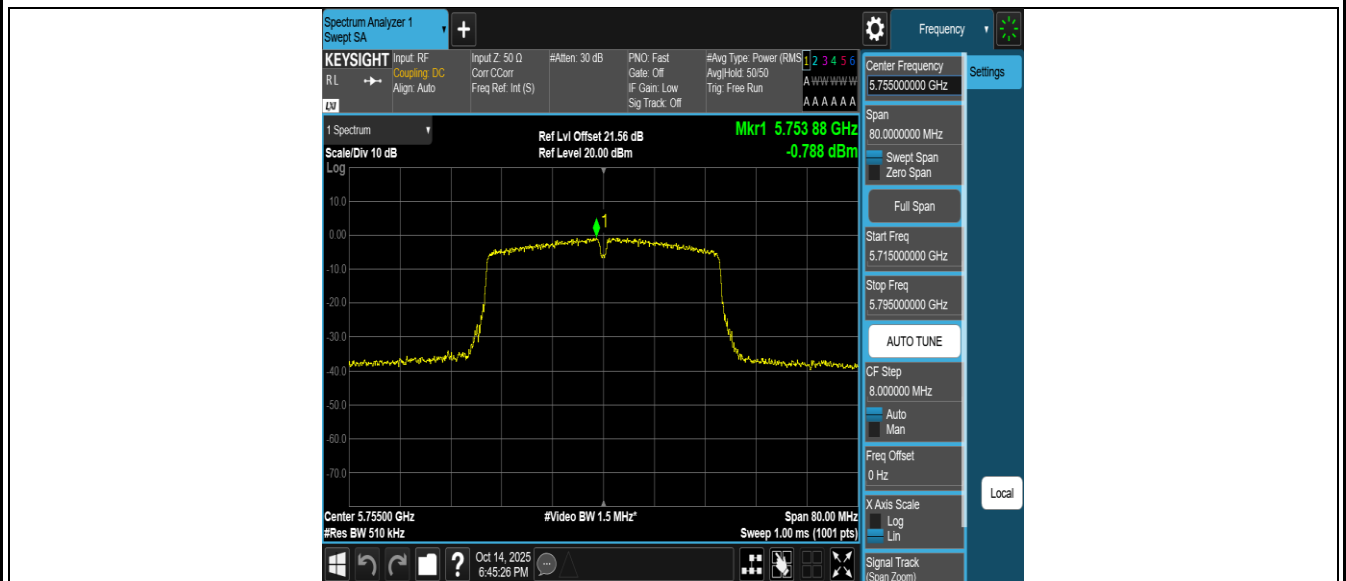
11N40MIMO Ant2 5755
