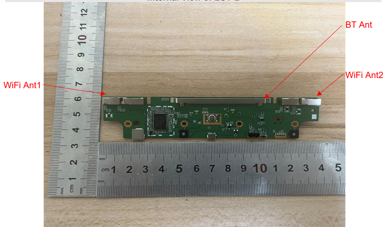
Internal View of EUT-2
