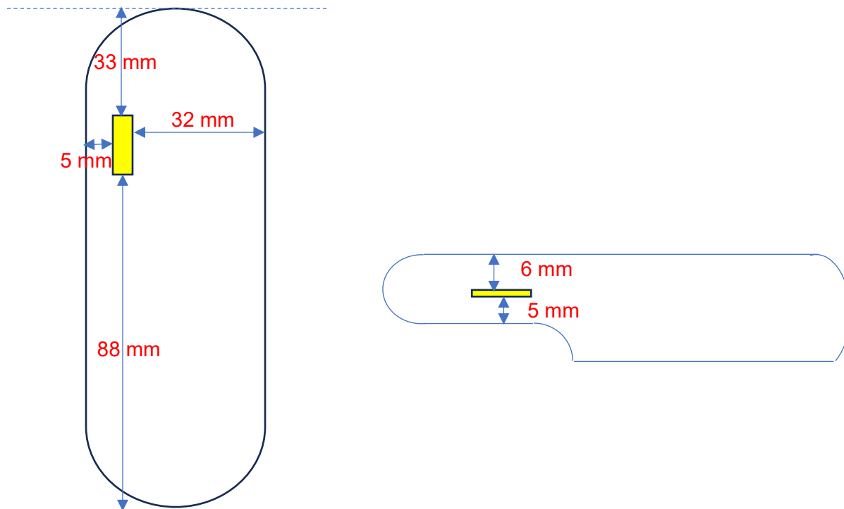
Antenna location diagram
