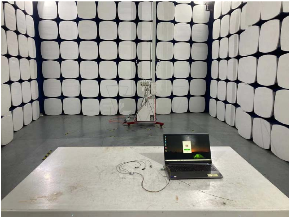
Radiated Emission Above 1G Test Photo
